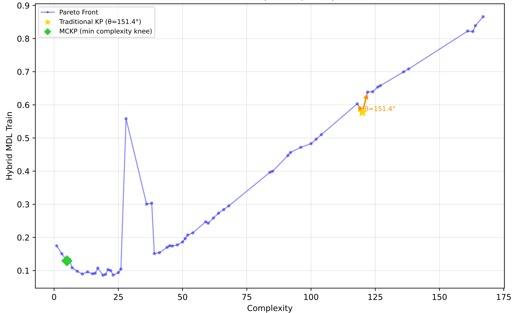
229_pwLinear - Run 26 - MVP - Hybrid MDL Train \lambda_1=0.50, \bar{\lambda}_2=0.00, \lambda_3=0.00 | Difficulty: 1.00 | Method: hmr
