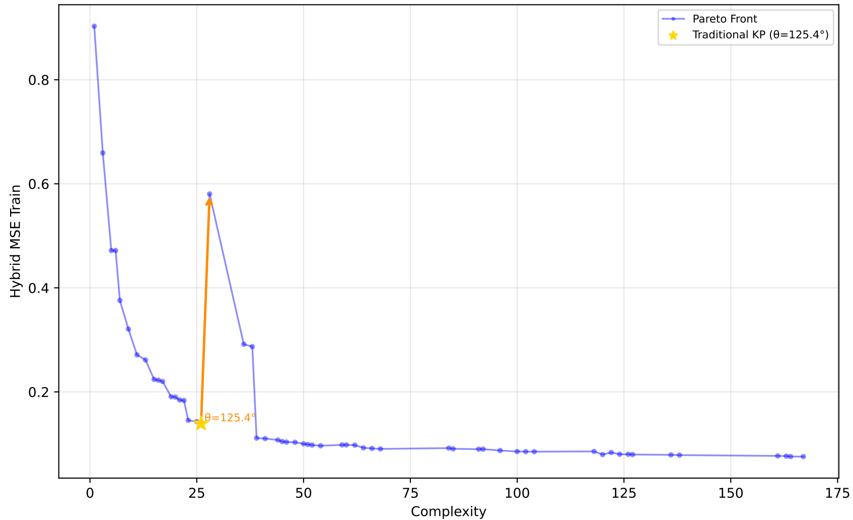
229_pwLinear - Run 26 - MVP - Hybrid MSE Train \lambda_1=0.50, \lambda_2=0.00, \lambda_3=0.00 | Difficulty: 1.00 | Method: hmr
