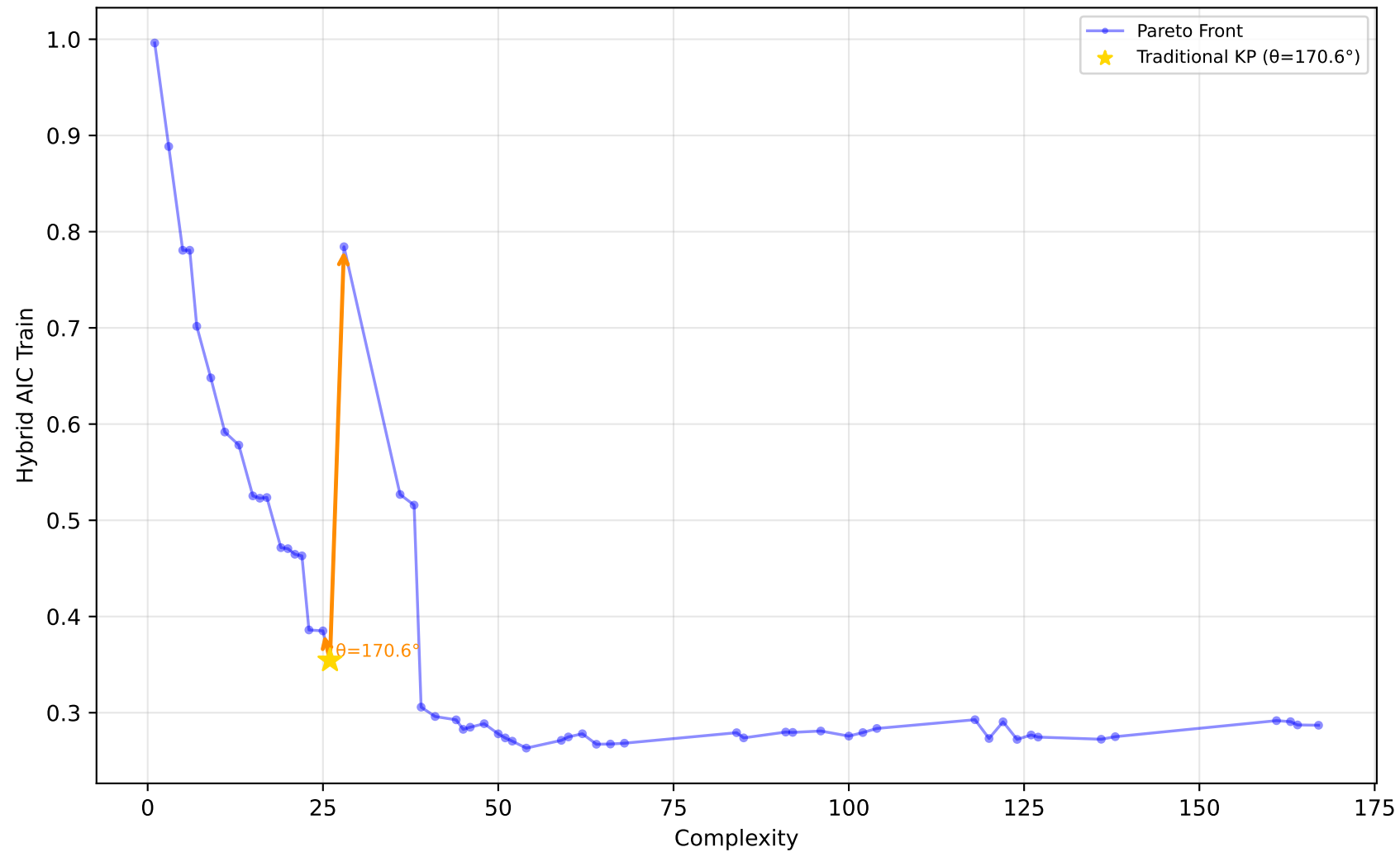
229_pwLinear - Run 26 - SVP - Hybrid AIC Train \lambda_1=0.50, \bar{\lambda}_2=0.10, \lambda_3=0.00 | Difficulty: 1.00 | Method: hmr
