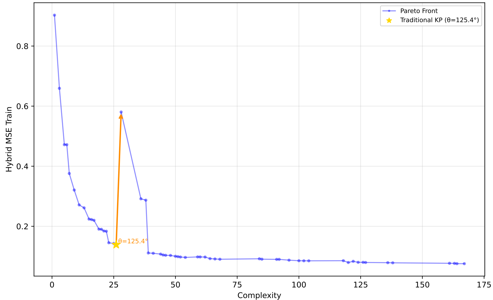
229_pwLinear - Run 26 - SVP - Hybrid MSE Train \lambda_1=0.50, \lambda_2=0.00, \lambda_3=0.00 | Difficulty: 1.00 | Method: hmr
