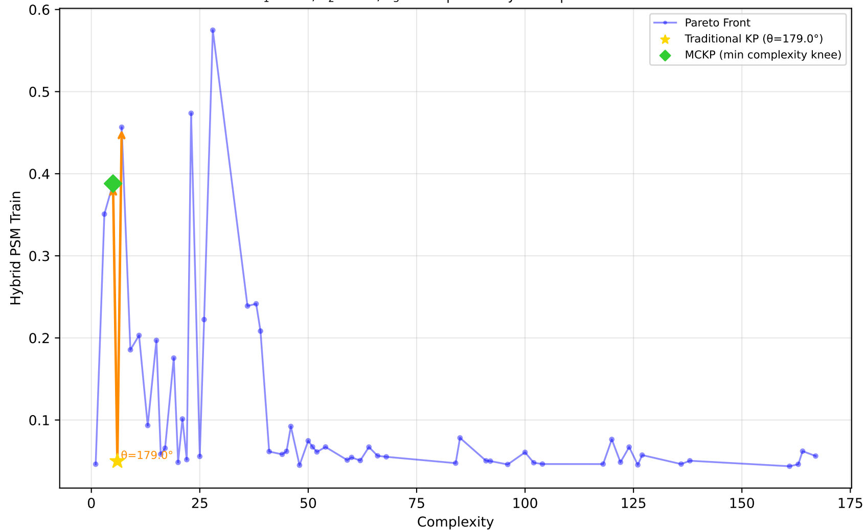
229_pwLinear - Run 26 - SVP - Hybrid PSM Train \lambda_1=0.50, \lambda_2=0.10, \lambda_3=0.00 | Difficulty: 1.00 | Method: hmr
