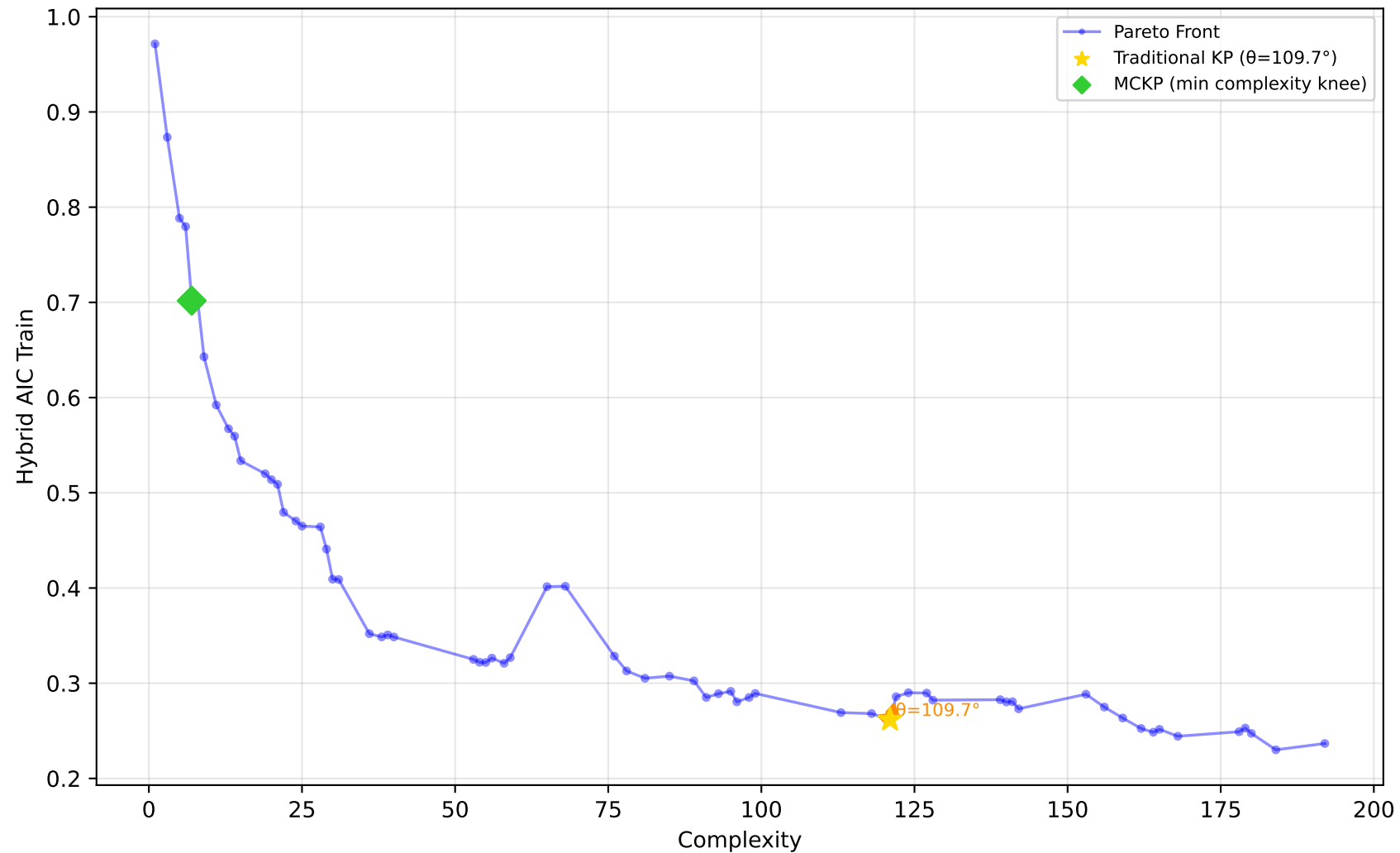
229_pwLinear - Run 27 - MVP - Hybrid AIC Train \lambda_1=0.50, \bar{\lambda}_2=0.00, \lambda_3=0.00 | Difficulty: 1.00 | Method: hmr
