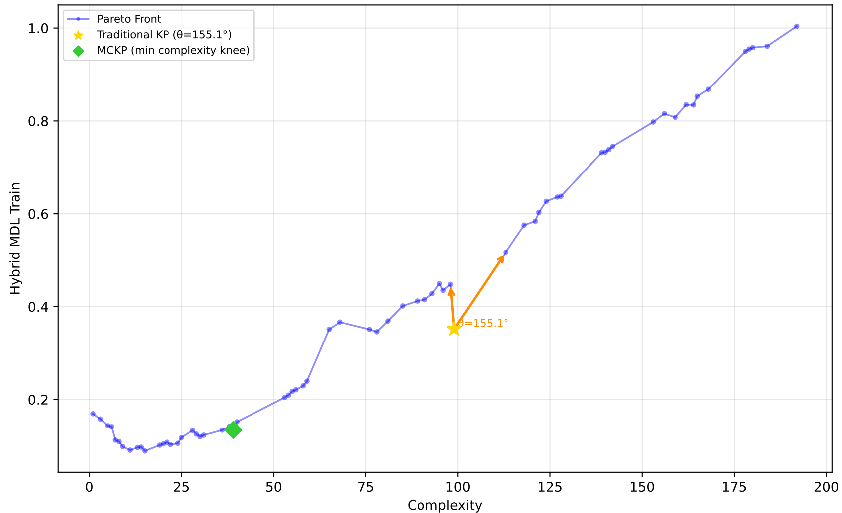
229_pwLinear - Run 27 - SVP - Hybrid MDL Train \lambda_1=0.50, \bar{\lambda}_2=0.00, \lambda_3=0.00 | Difficulty: 1.00 | Method: hmr
