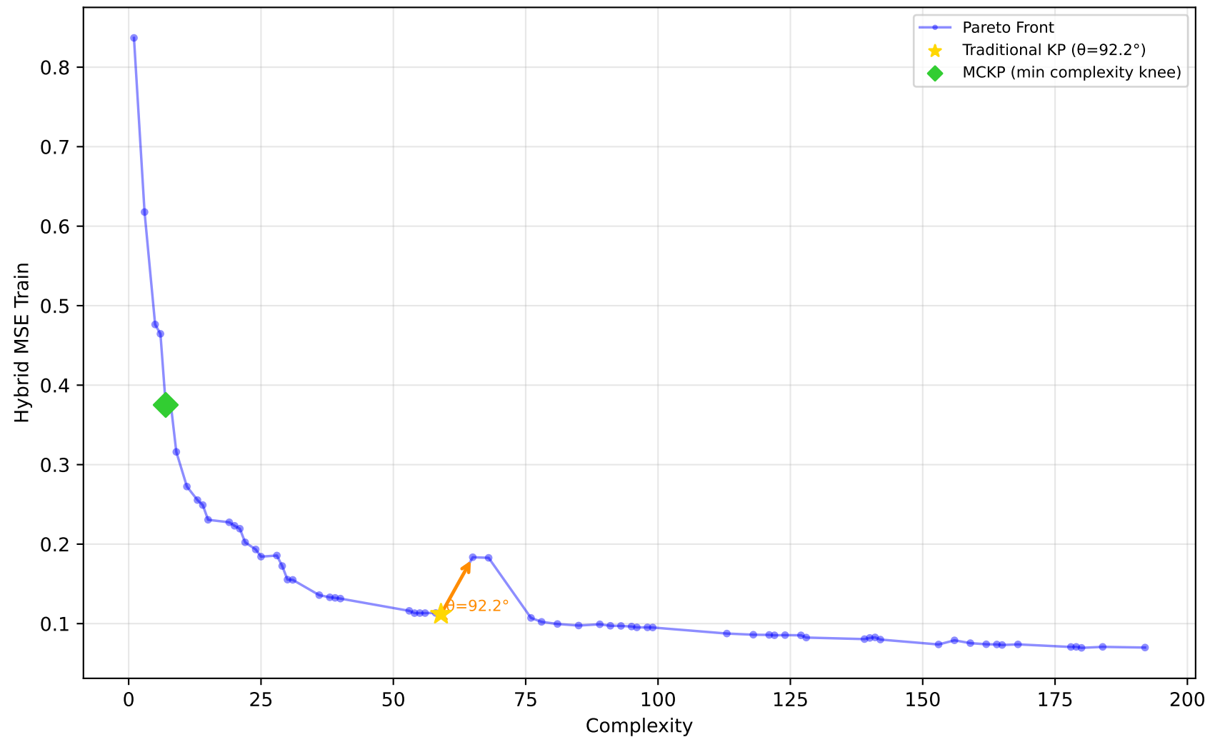
229_pwLinear - Run 27 - SVP - Hybrid MSE Train \lambda_1=0.50, \bar{\lambda}_2=0.00, \lambda_3=0.00 | Difficulty: 1.00 | Method: hmr
