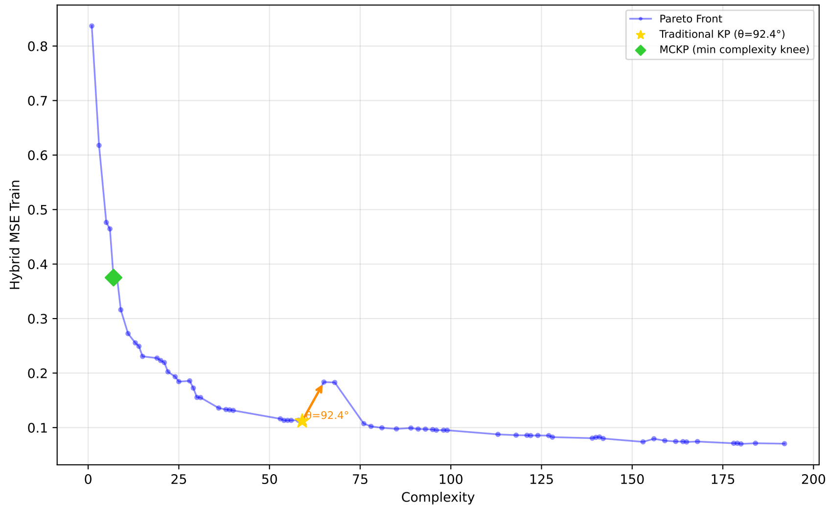
229_pwLinear - Run 27 - SVP - Hybrid MSE Train \lambda_1=0.50, \bar{\lambda}_2=0.10, \lambda_3=0.00 | Difficulty: 1.00 | Method: hmr
