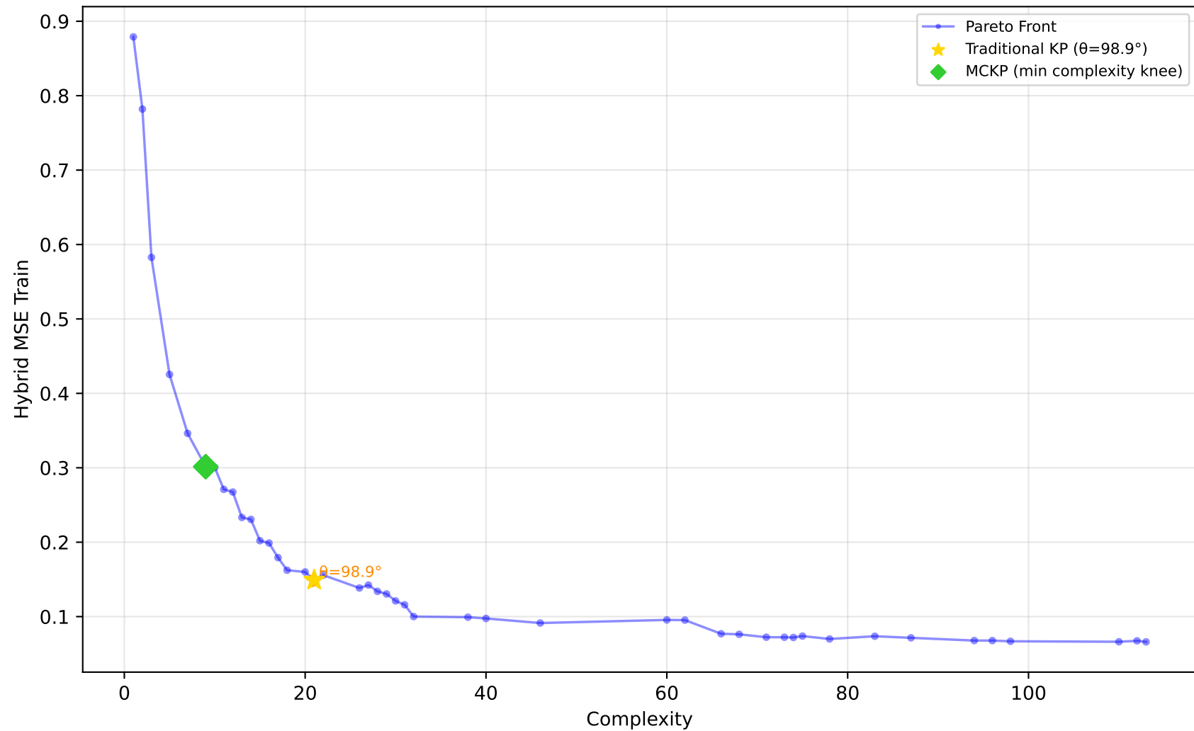
229_pwLinear - Run 28 - MVP - Hybrid MSE Train \lambda_1=0.50, \lambda_2=0.00, \lambda_3=0.00 | Difficulty: 1.00 | Method: hmr
