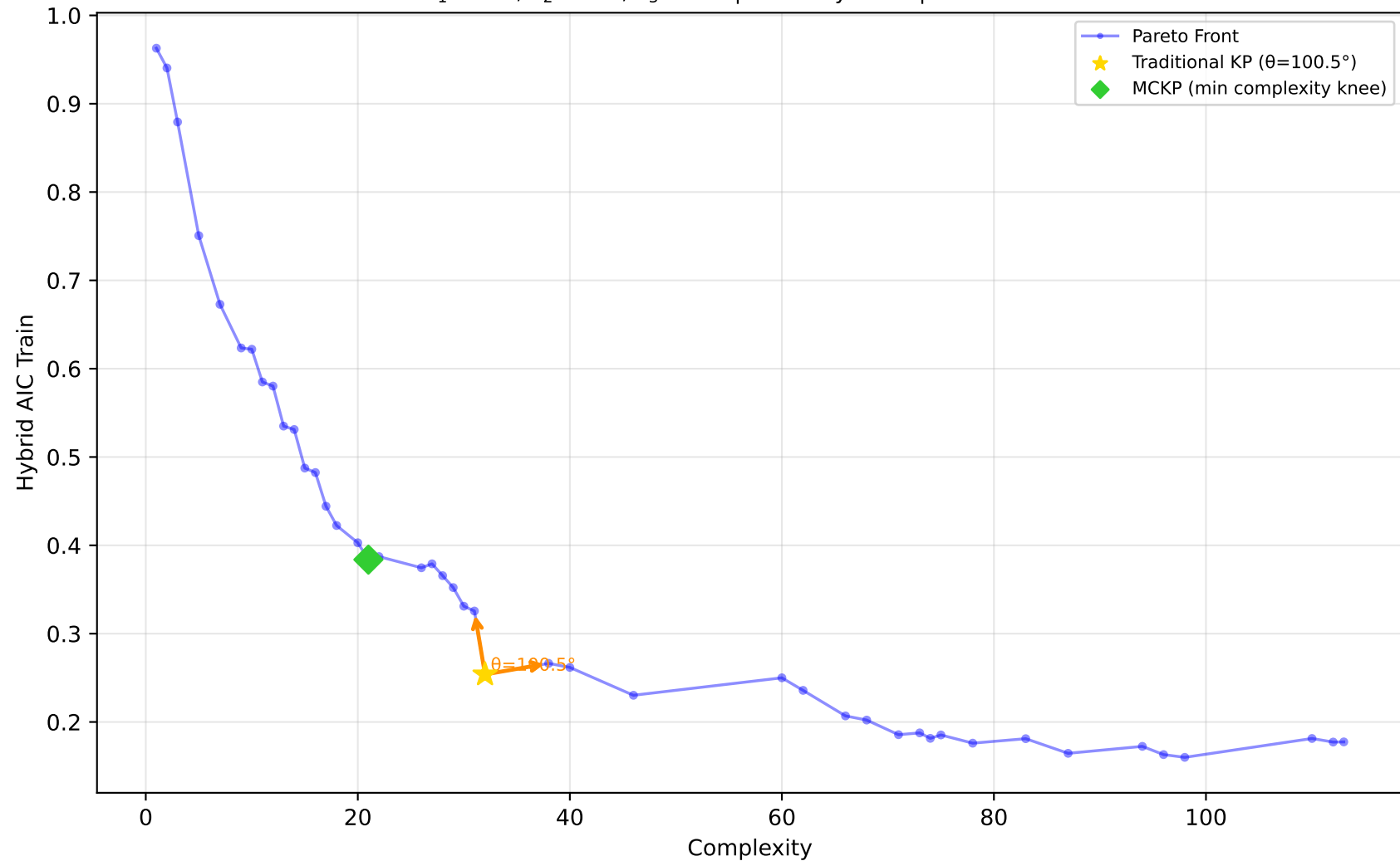
229_pwLinear - Run 28 - SVP - Hybrid AIC Train \lambda_1=0.50, \lambda_2=0.00, \lambda_3=0.00 | Difficulty: 1.00 | Method: hmr
