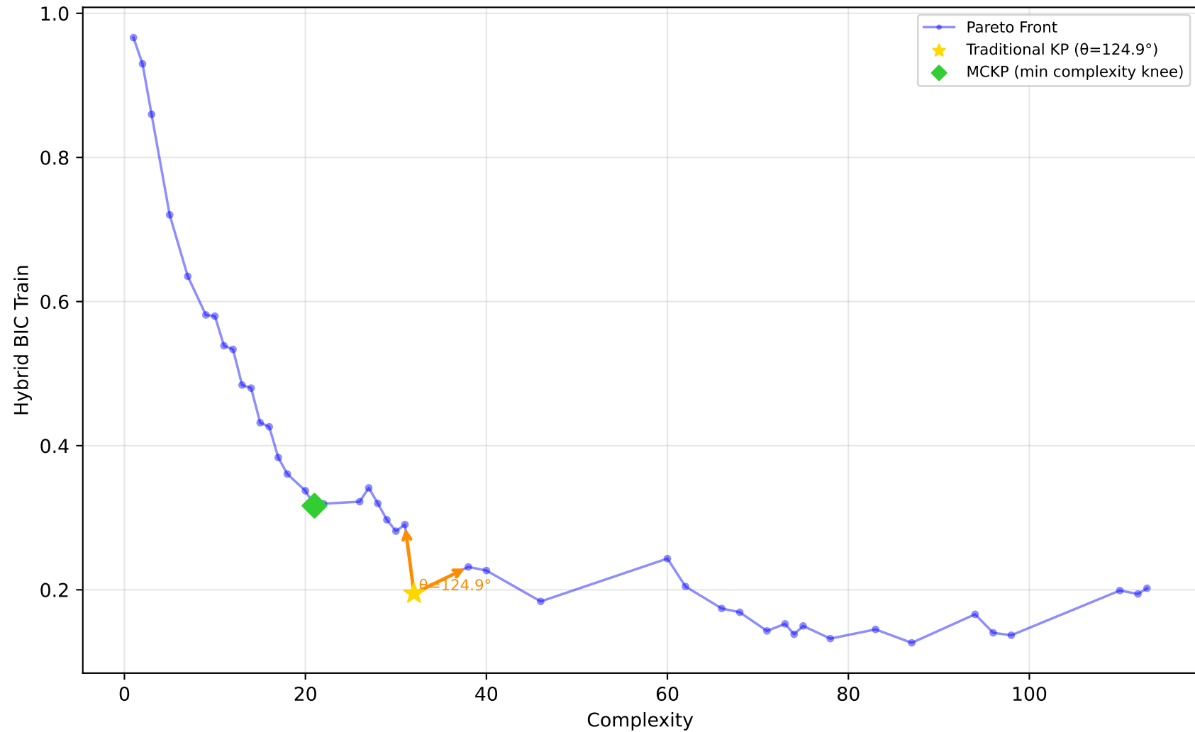
229_pwLinear - Run 28 - SVP - Hybrid BIC Train \lambda_1=0.50, \lambda_2=0.00, \lambda_3=0.00 | Difficulty: 1.00 | Method: hmr
