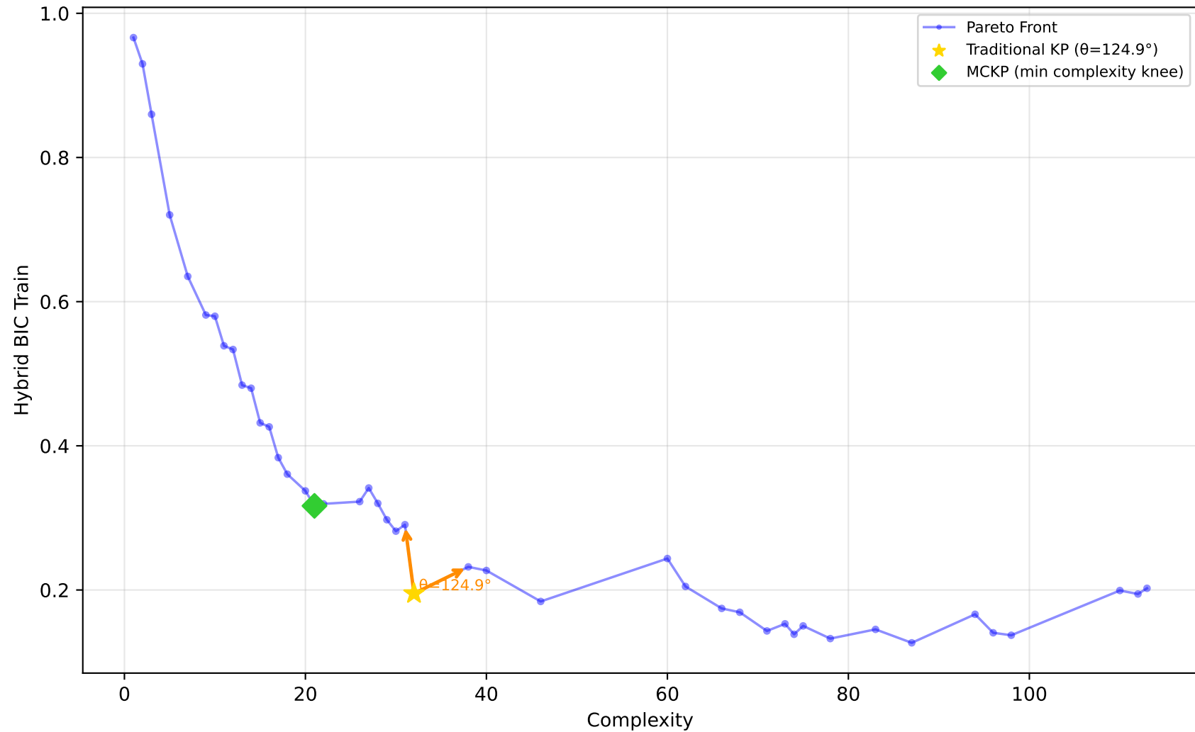
229_pwLinear - Run 28 - SVP - Hybrid BIC Train \lambda_1=0.50, \lambda_2=0.10, \lambda_3=0.00 | Difficulty: 1.00 | Method: hmr
