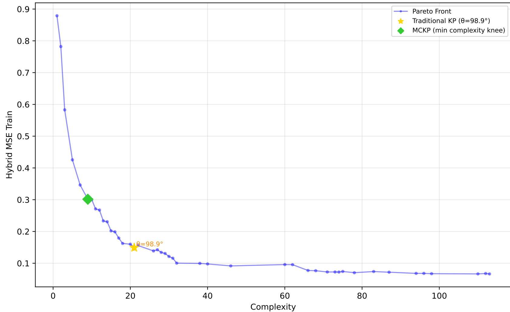
229_pwLinear - Run 28 - SVP - Hybrid MSE Train \lambda_1=0.50, \lambda_2=0.10, \lambda_3=0.00 | Difficulty: 1.00 | Method: hmr
