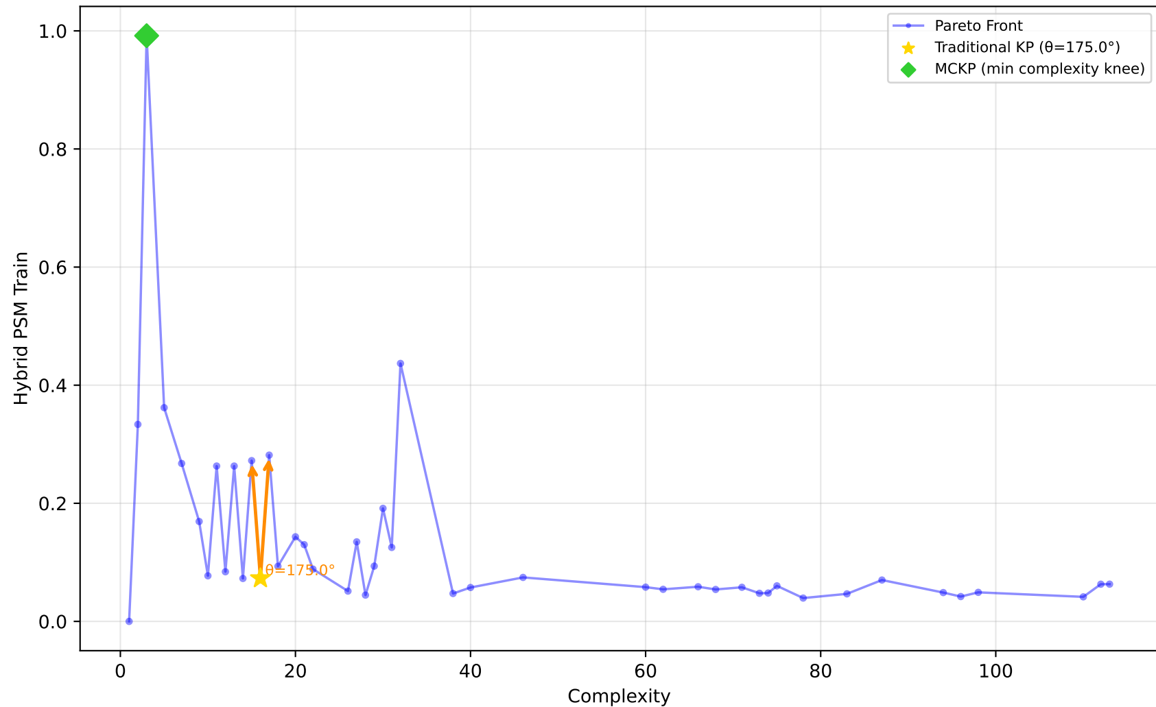
229_pwLinear - Run 28 - SVP - Hybrid PSM Train \lambda_1=0.50, \lambda_2=0.00, \lambda_3=0.00 | Difficulty: 1.00 | Method: hmr
