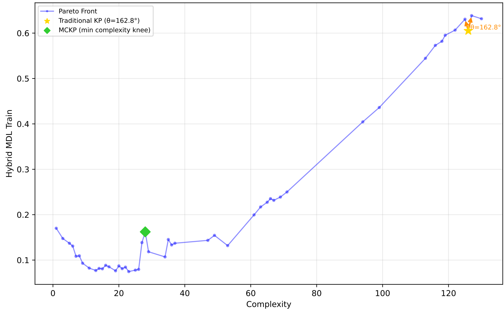
229_pwLinear - Run 29 - MVP - Hybrid MDL Train \lambda_1=0.50, \lambda_2=0.00, \lambda_3=0.00 | Difficulty: 1.00 | Method: hmr
