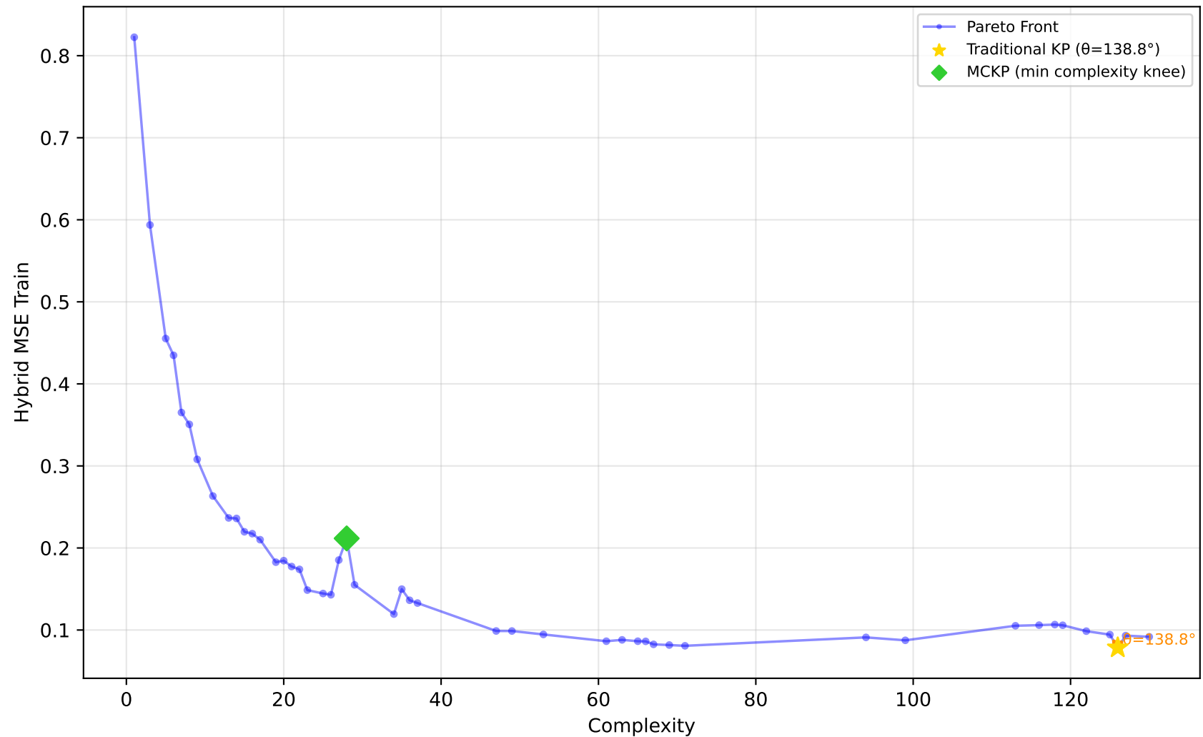
229_pwLinear - Run 29 - MVP - Hybrid MSE Train \lambda_1=0.50, \lambda_2=0.00, \lambda_3=0.00 | Difficulty: 1.00 | Method: hmr
