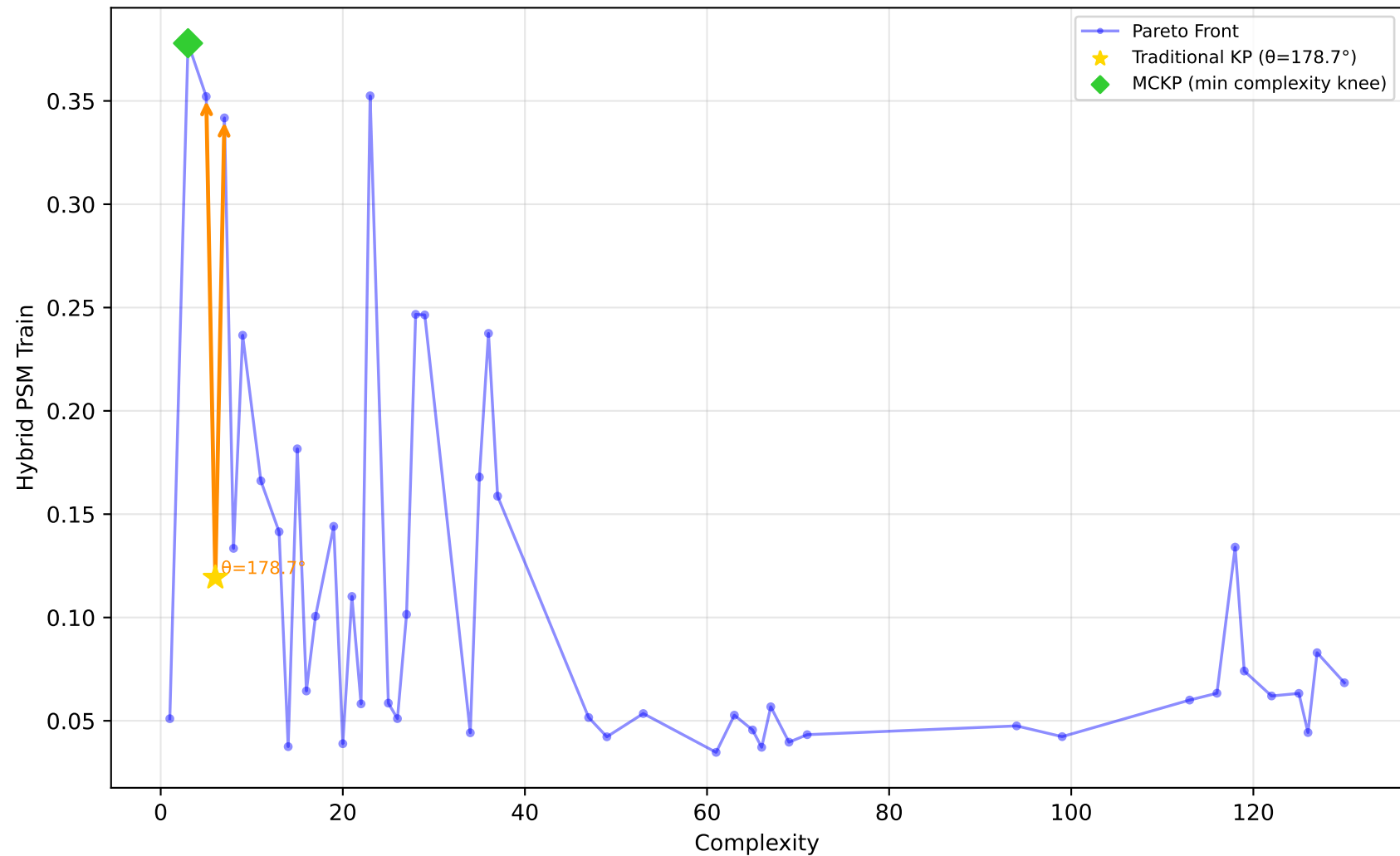
229_pwLinear - Run 29 - MVP - Hybrid PSM Train \lambda_1=0.50, \bar{\lambda}_2=0.00, \lambda_3=0.00 | Difficulty: 1.00 | Method: hmr
