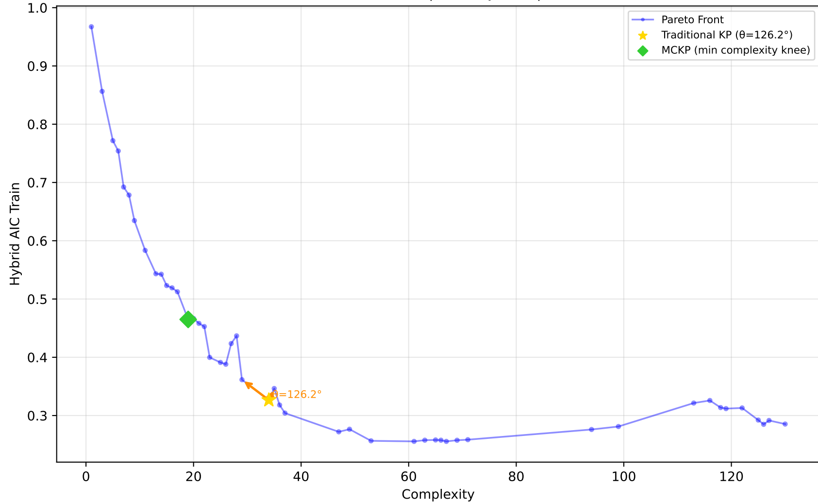
229_pwLinear - Run 29 - SVP - Hybrid AIC Train \lambda_1=0.50, \bar{\lambda}_2=0.00, \lambda_3=0.00 | Difficulty: 1.00 | Method: hmr
