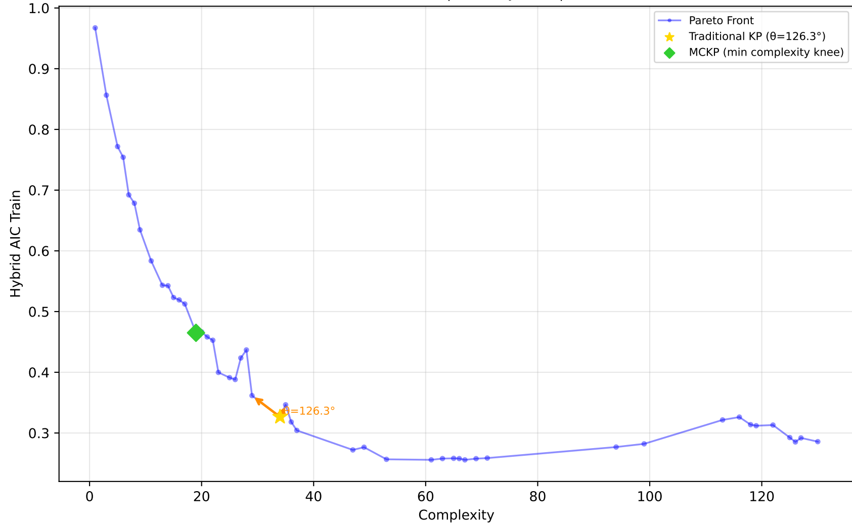
229_pwLinear - Run 29 - SVP - Hybrid AIC Train \lambda_1=0.50, \lambda_2=0.10, \lambda_3=0.00 | Difficulty: 1.00 | Method: hmr
