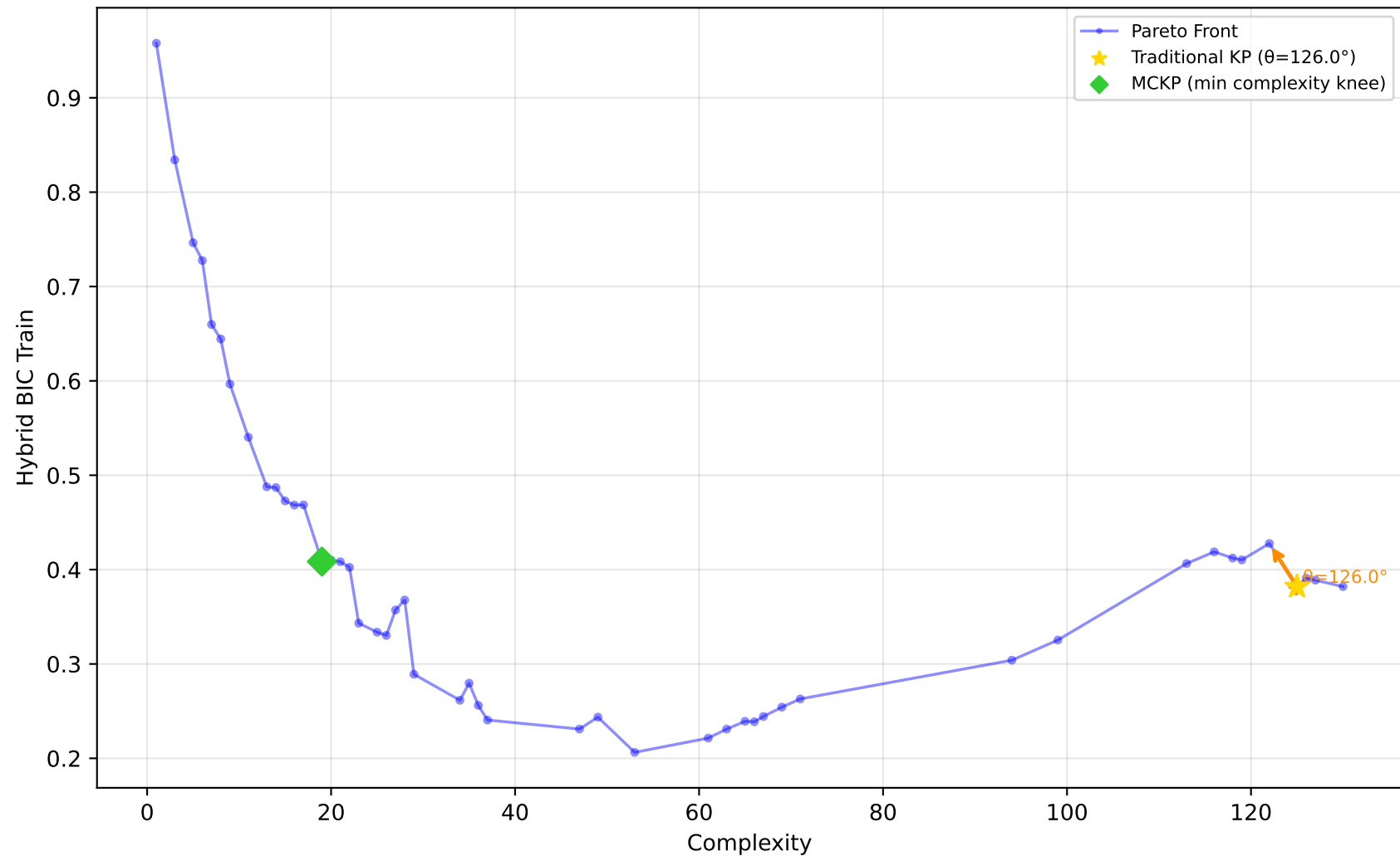
229_pwLinear - Run 29 - SVP - Hybrid BIC Train \lambda_1=0.50, \lambda_2=0.00, \lambda_3=0.00 | Difficulty: 1.00 | Method: hmr
