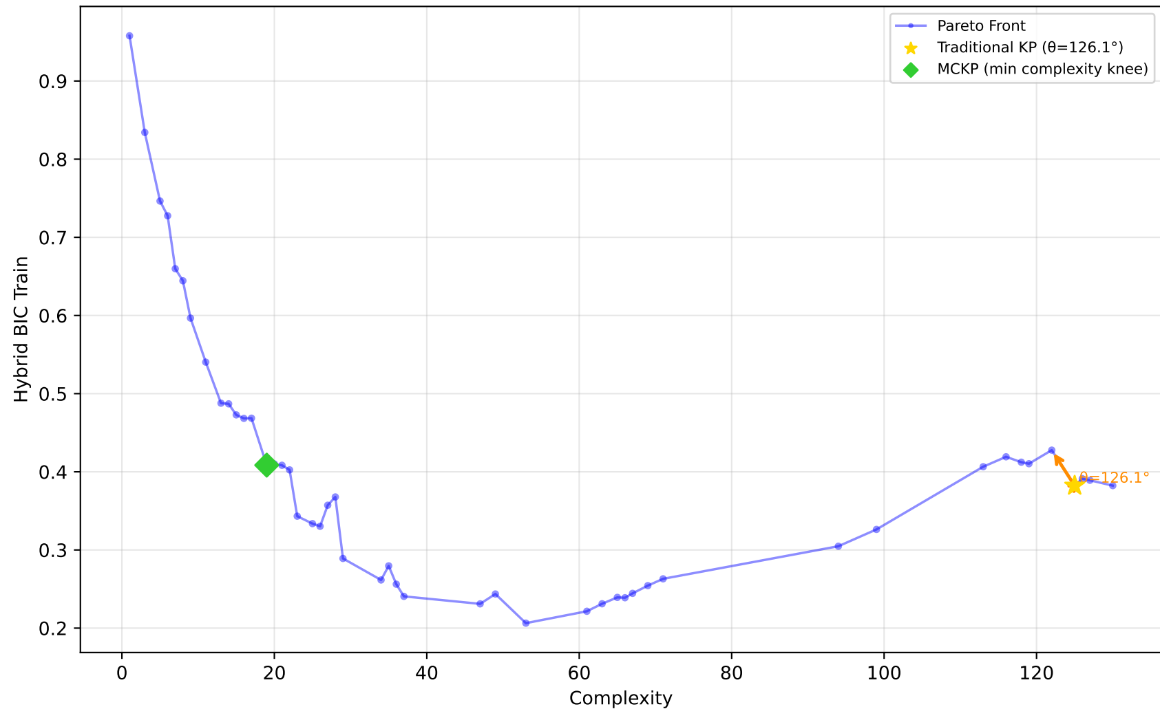
229_pwLinear - Run 29 - SVP - Hybrid BIC Train \lambda_1=0.50, \lambda_2=0.10, \lambda_3=0.00 | Difficulty: 1.00 | Method: hmr
