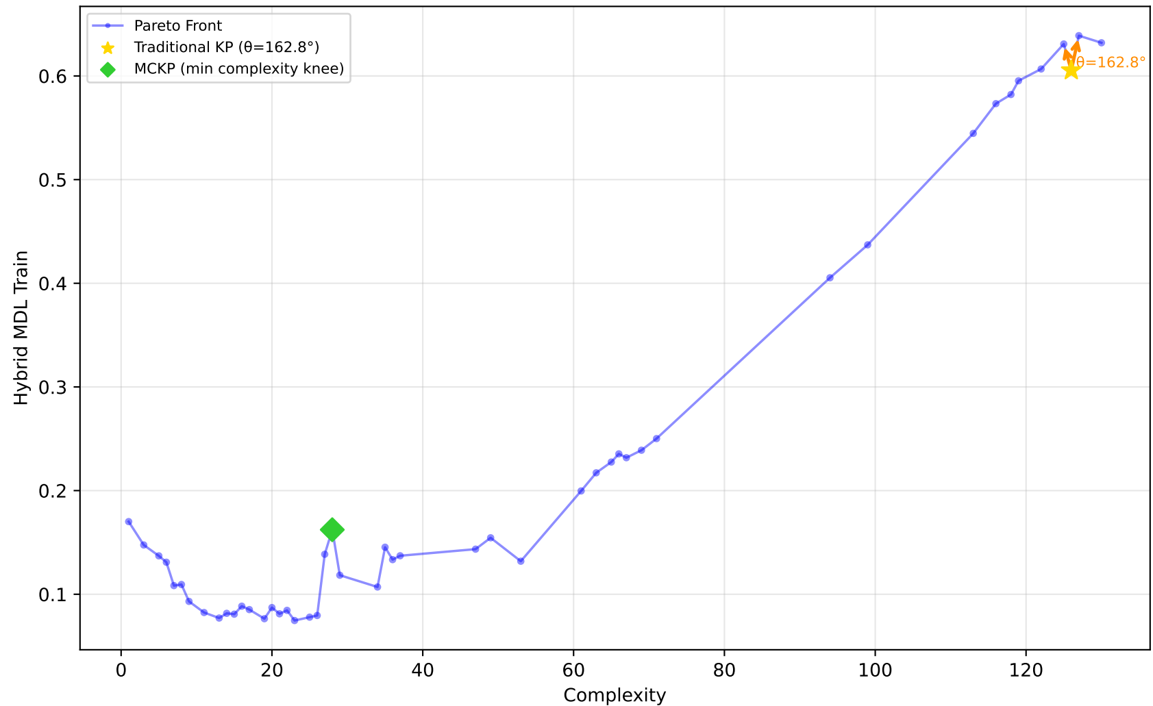
229_pwLinear - Run 29 - SVP - Hybrid MDL Train \lambda_1=0.50, \lambda_2=0.10, \lambda_3=0.00 | Difficulty: 1.00 | Method: hmr
