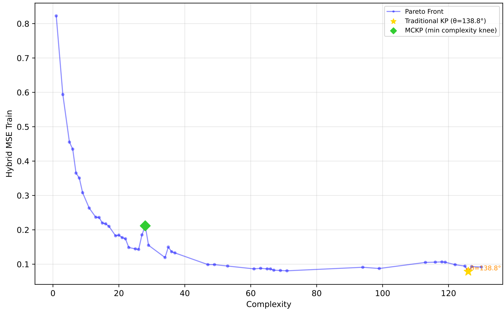
229_pwLinear - Run 29 - SVP - Hybrid MSE Train \lambda_1=0.50, \lambda_2=0.00, \lambda_3=0.00 | Difficulty: 1.00 | Method: hmr
