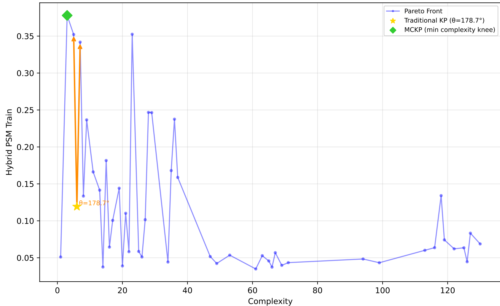
229_pwLinear - Run 29 - SVP - Hybrid PSM Train \lambda_1=0.50, \bar{\lambda}_2=0.10, \lambda_3=0.00 | Difficulty: 1.00 | Method: hmr
