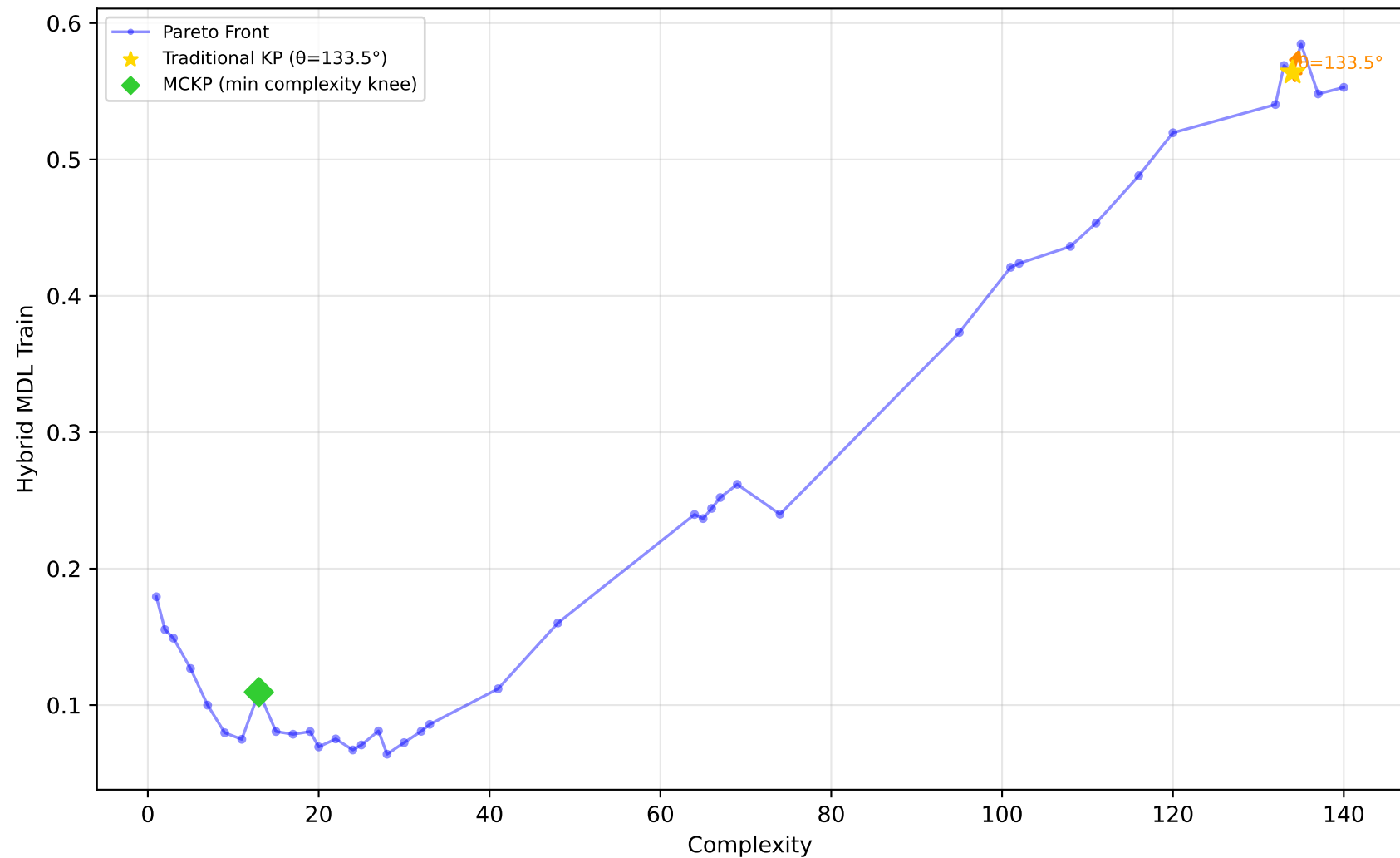
229_pwLinear - Run 2 - MVP - Hybrid MDL Train \lambda_1=0.50, \lambda_2=0.00, \lambda_3=0.00 | Difficulty: 1.00 | Method: hmr
