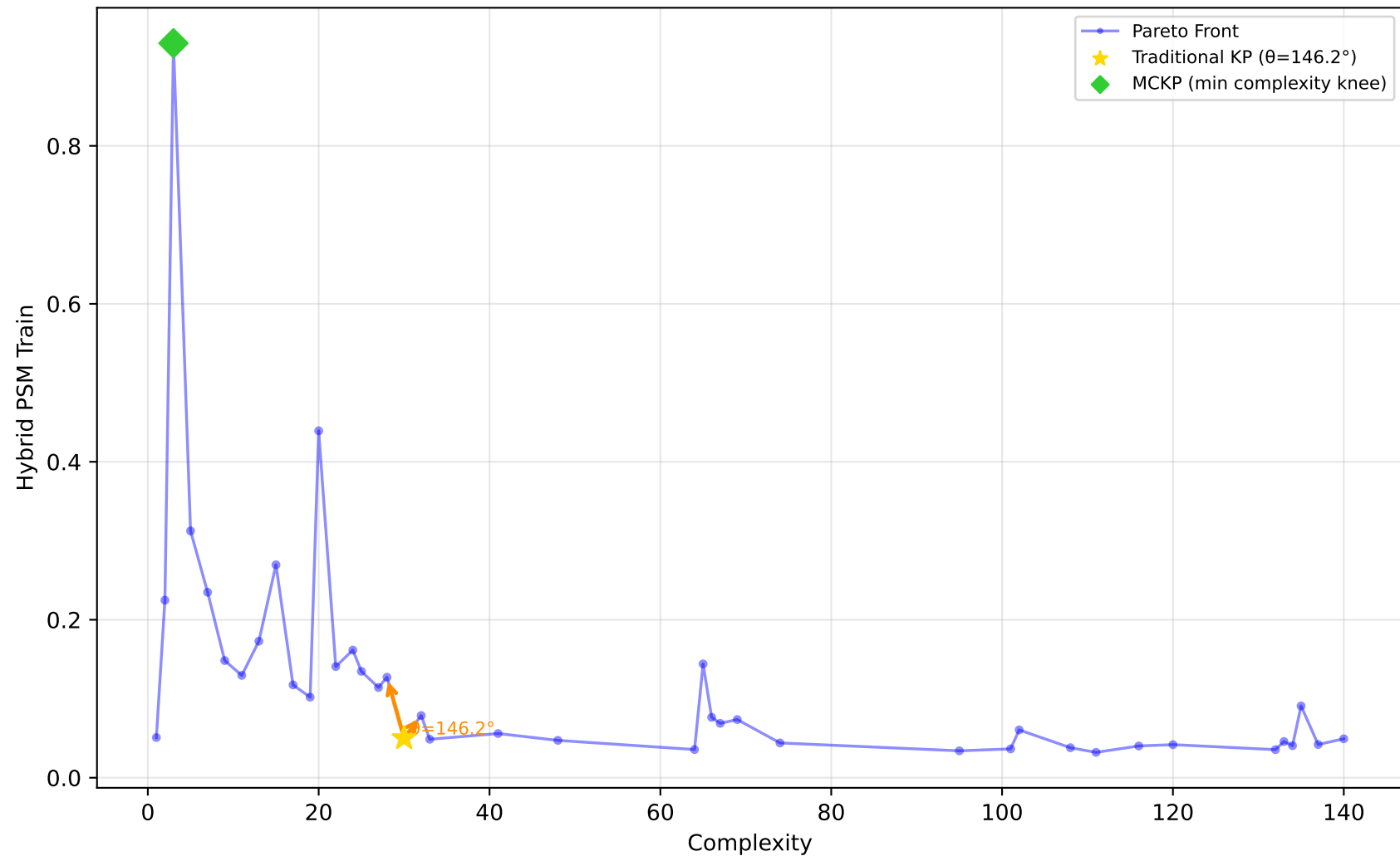
229_pwLinear - Run 2 - MVP - Hybrid PSM Train \lambda_1=0.50, \lambda_2=0.00, \lambda_3=0.00 | Difficulty: 1.00 | Method: hmr
