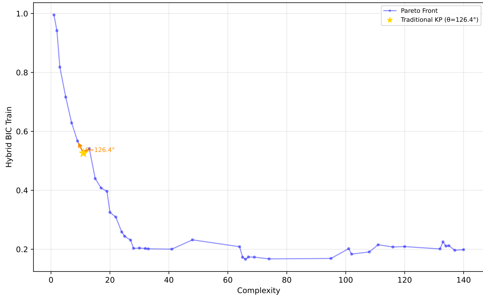
229_pwLinear - Run 2 - SVP - Hybrid BIC Train \lambda_1=0.50, \lambda_2=0.00, \lambda_3=0.00 | Difficulty: 1.00 | Method: hmr
