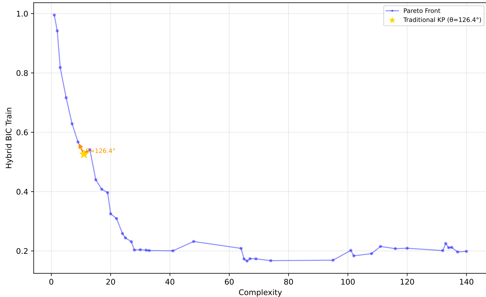
229_pwLinear - Run 2 - SVP - Hybrid BIC Train \lambda_1=0.50, \lambda_2=0.10, \lambda_3=0.00 | Difficulty: 1.00 | Method: hmr
