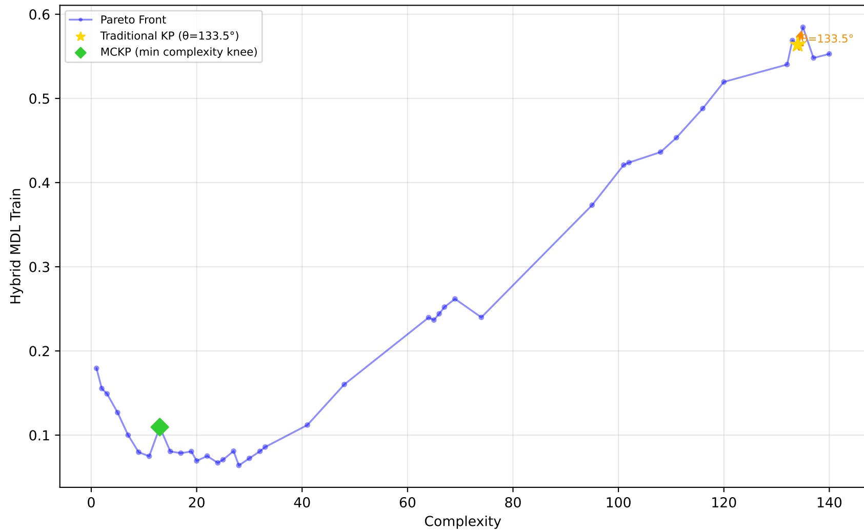
229_pwLinear - Run 2 - SVP - Hybrid MDL Train \lambda_1=0.50, \bar{\lambda}_2=0.00, \lambda_3=0.00 | Difficulty: 1.00 | Method: hmr
