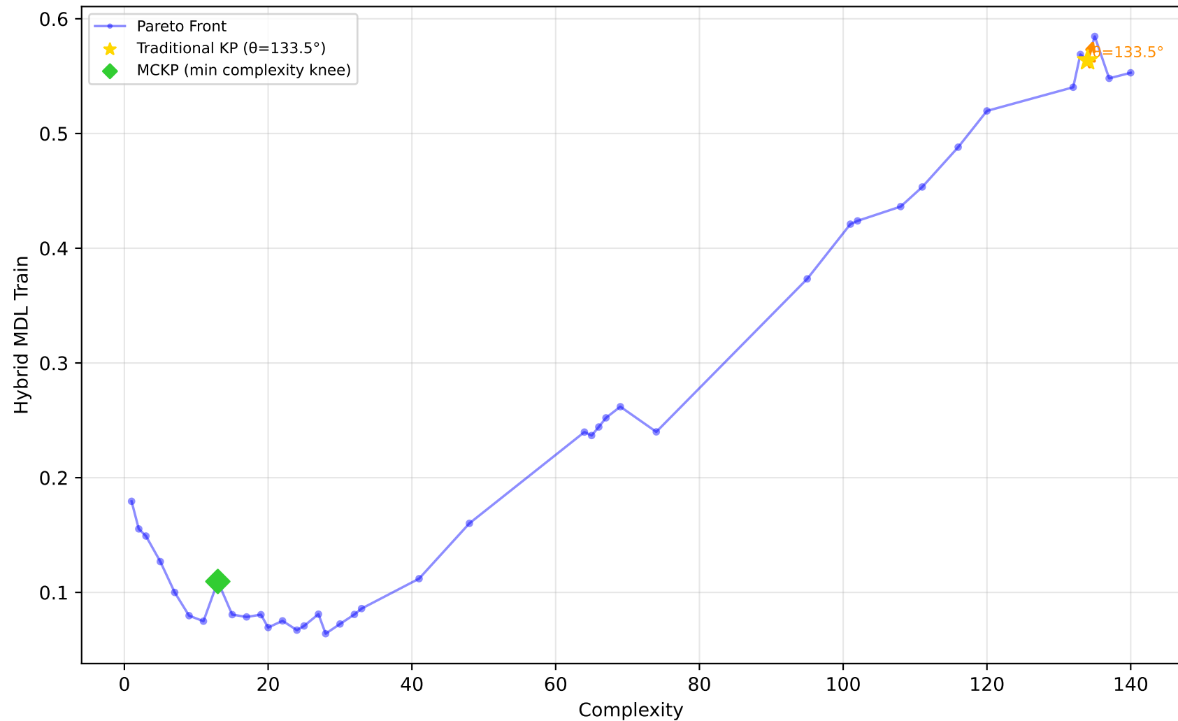
229_pwLinear - Run 2 - SVP - Hybrid MDL Train \lambda_1=0.50, \bar{\lambda}_2=0.10, \lambda_3=0.00 | Difficulty: 1.00 | Method: hmr
