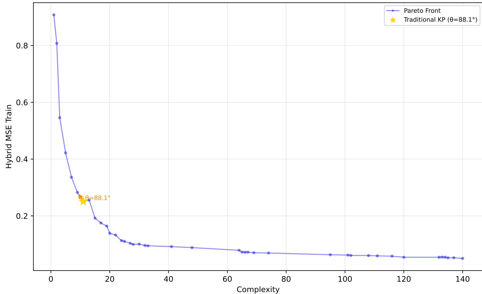
229_pwLinear - Run 2 - SVP - Hybrid MSE Train \lambda_1=0.50, \lambda_2=0.10, \lambda_3=0.00 | Difficulty: 1.00 | Method: hmr
