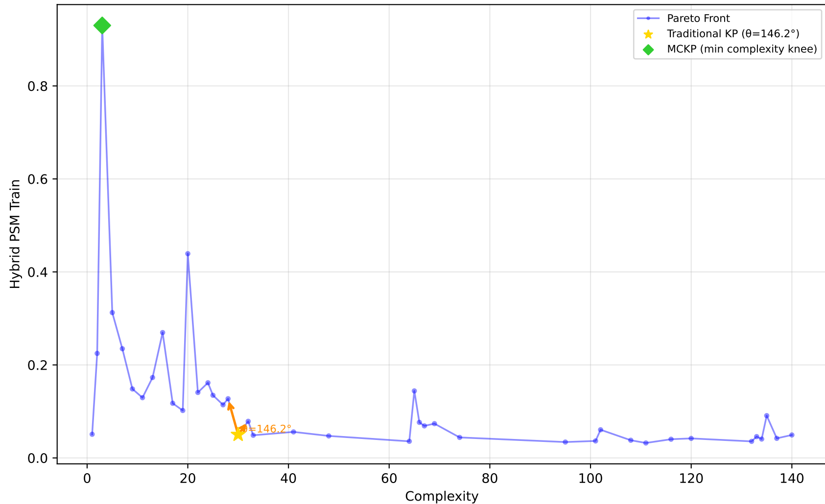
229_pwLinear - Run 2 - SVP - Hybrid PSM Train \lambda_1=0.50, \lambda_2=0.10, \lambda_3=0.00 | Difficulty: 1.00 | Method: hmr
