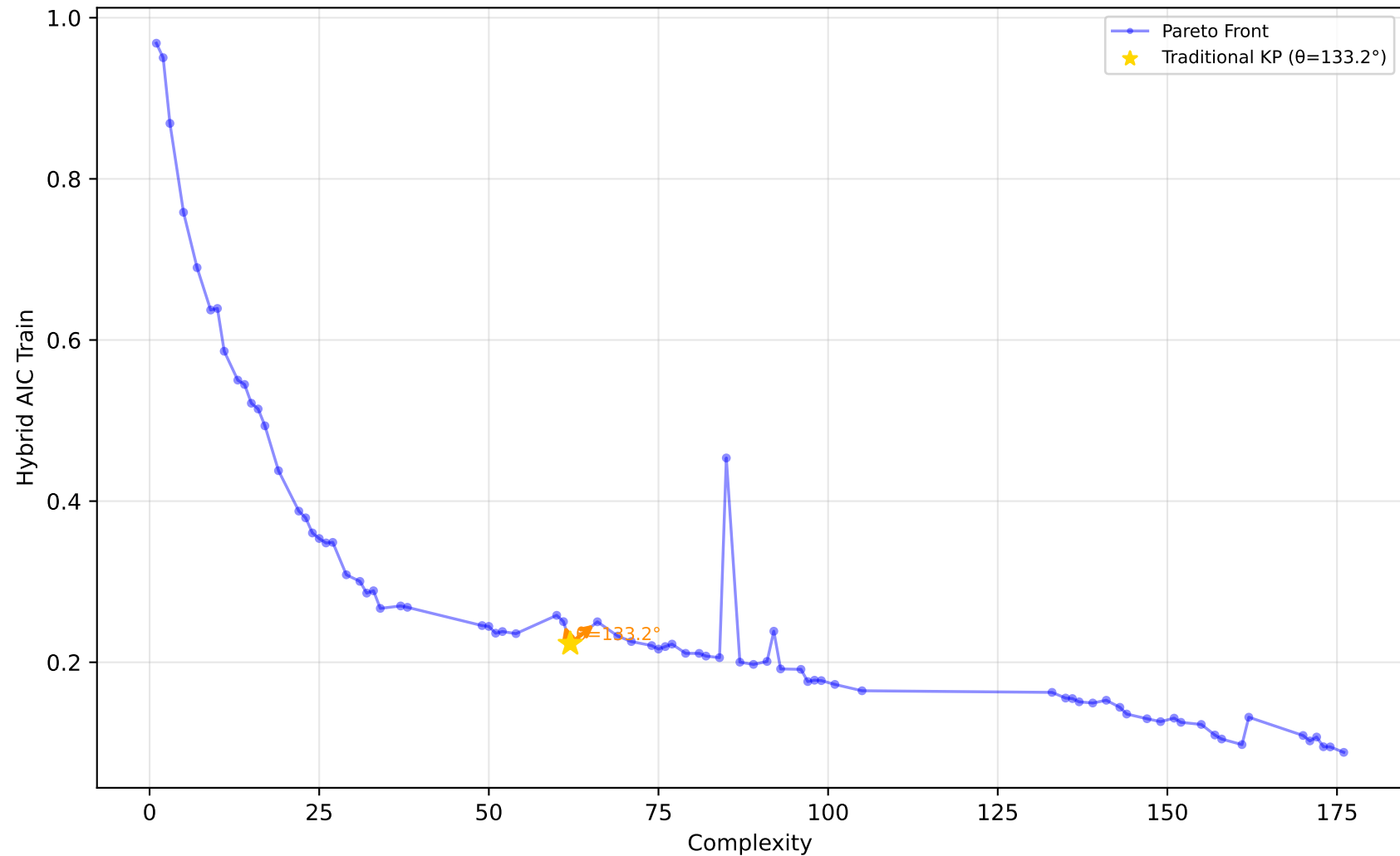
229_pwLinear - Run 30 - MVP - Hybrid AIC Train \lambda_1=0.50, \lambda_2=0.00, \lambda_3=0.00 | Difficulty: 1.00 | Method: hmr
