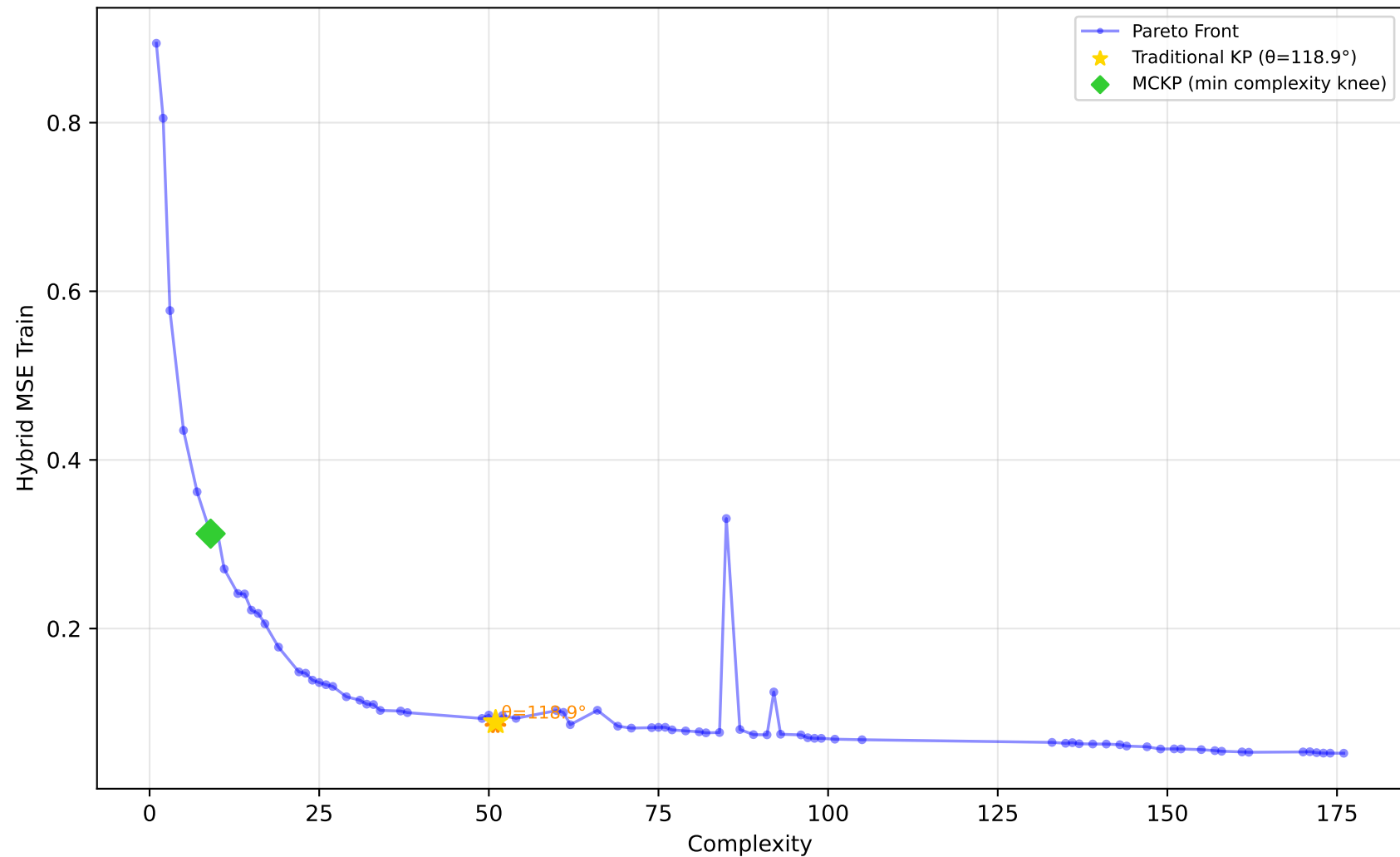
229_pwLinear - Run 30 - MVP - Hybrid MSE Train \lambda_1=0.50, \lambda_2=0.00, \lambda_3=0.00 | Difficulty: 1.00 | Method: hmr
