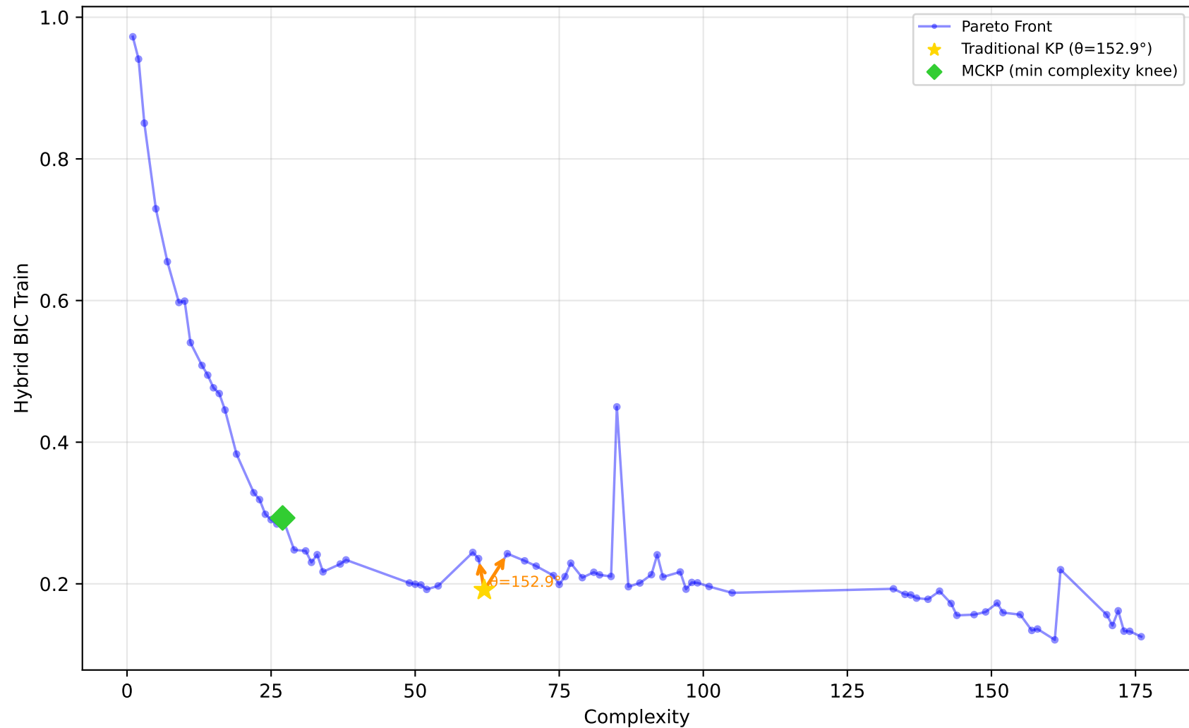
229_pwLinear - Run 30 - SVP - Hybrid BIC Train \lambda_1=0.50, \lambda_2=0.10, \lambda_3=0.00 | Difficulty: 1.00 | Method: hmr
