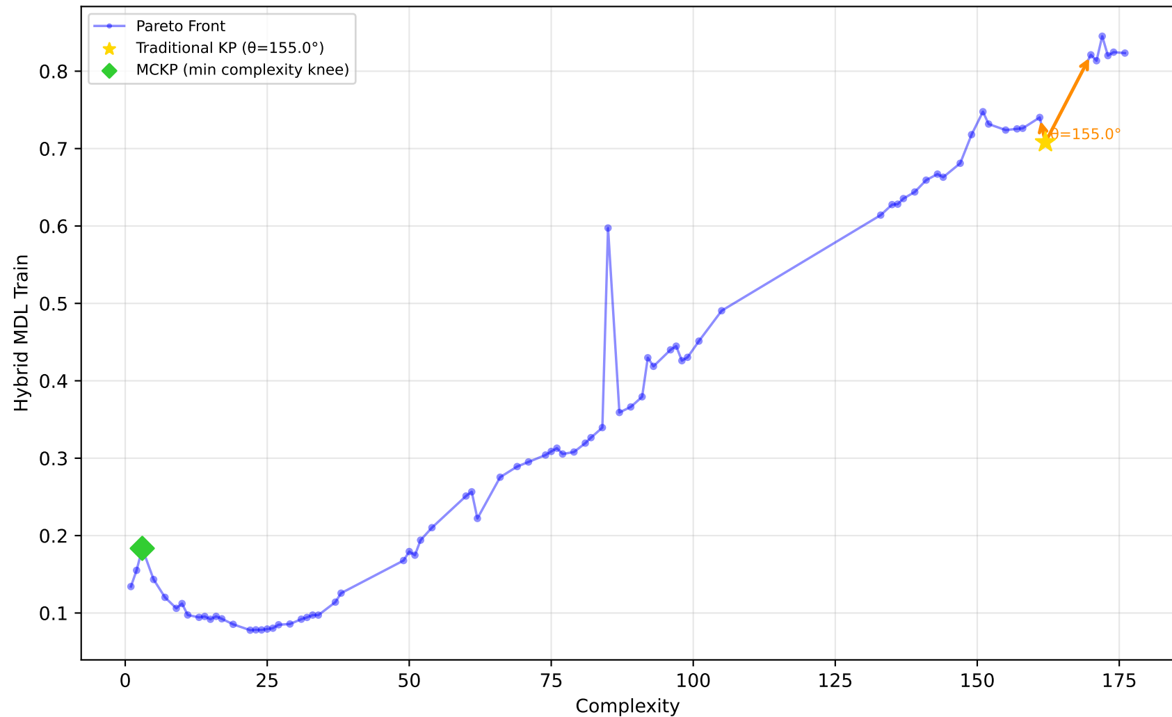
229_pwLinear - Run 30 - SVP - Hybrid MDL Train \lambda_1=0.50, \lambda_2=0.00, \lambda_3=0.00 | Difficulty: 1.00 | Method: hmr
