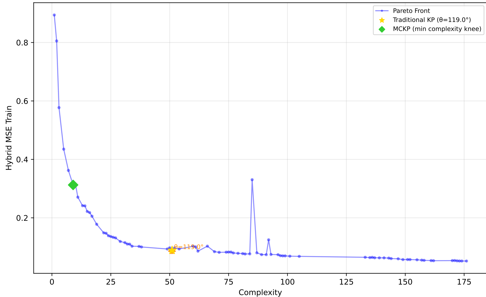
229_pwLinear - Run 30 - SVP - Hybrid MSE Train \lambda_1=0.50, \lambda_2=0.10, \lambda_3=0.00 | Difficulty: 1.00 | Method: hmr
