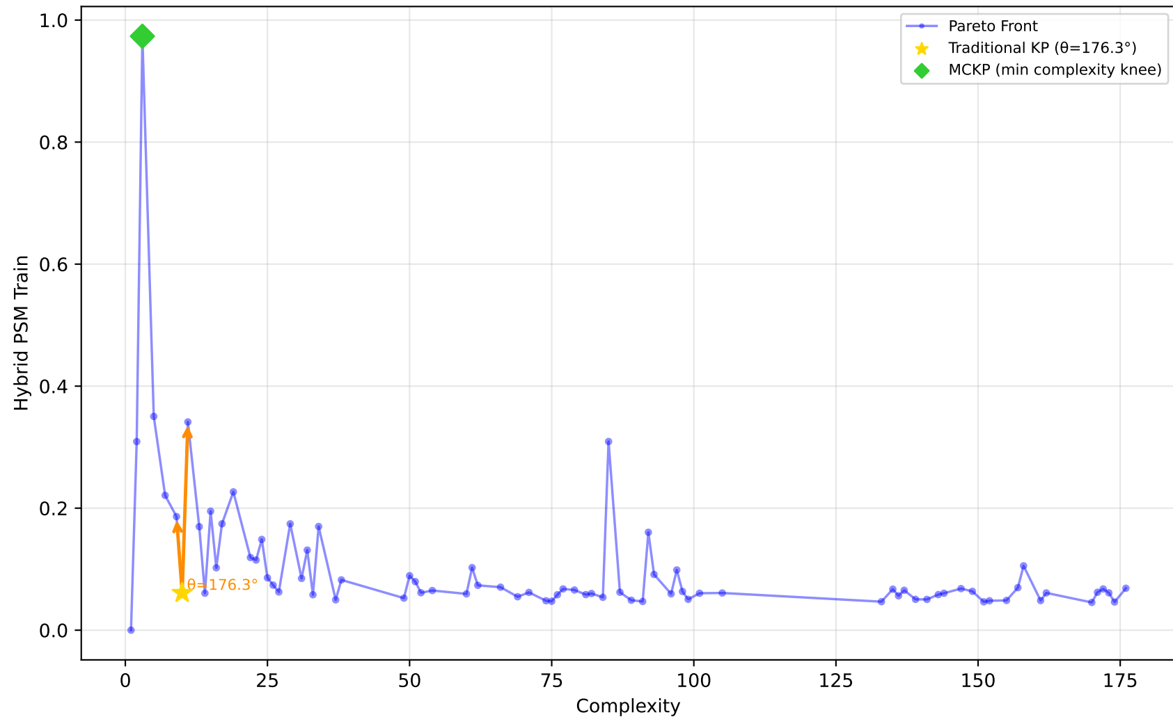
229_pwLinear - Run 30 - SVP - Hybrid PSM Train \lambda_1=0.50, \lambda_2=0.00, \lambda_3=0.00 | Difficulty: 1.00 | Method: hmr
