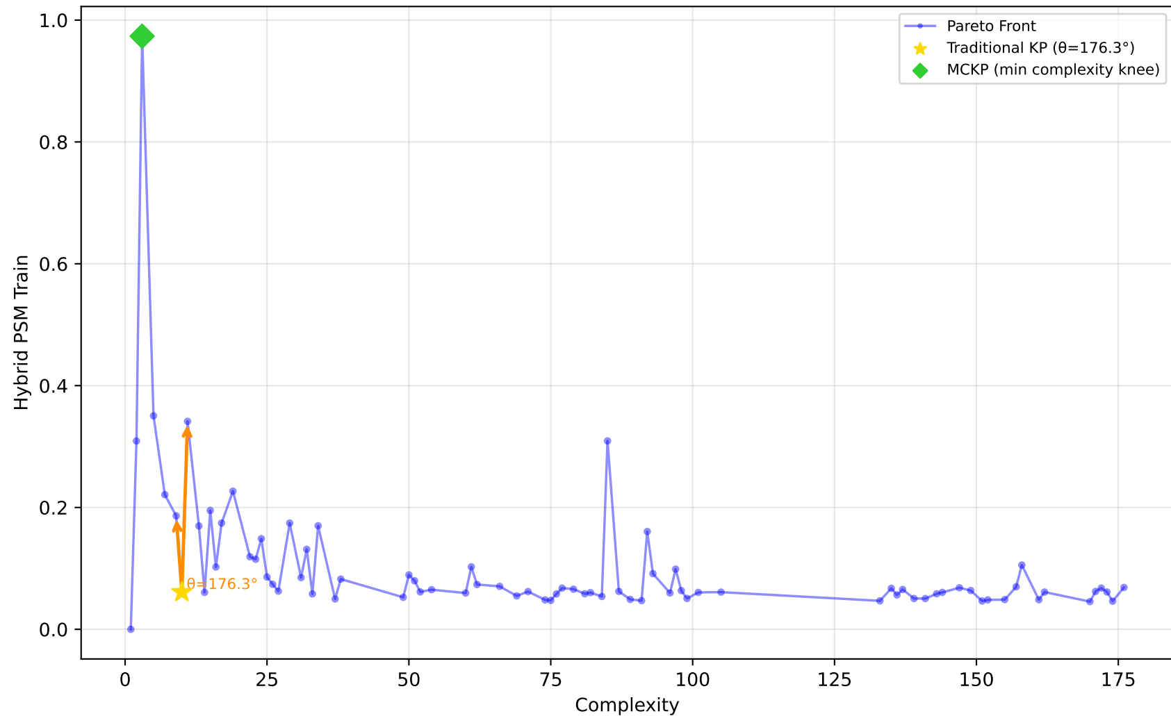
229_pwLinear - Run 30 - SVP - Hybrid PSM Train \lambda_1=0.50, \bar{\lambda}_2=0.10, \lambda_3=0.00 | Difficulty: 1.00 | Method: hmr
