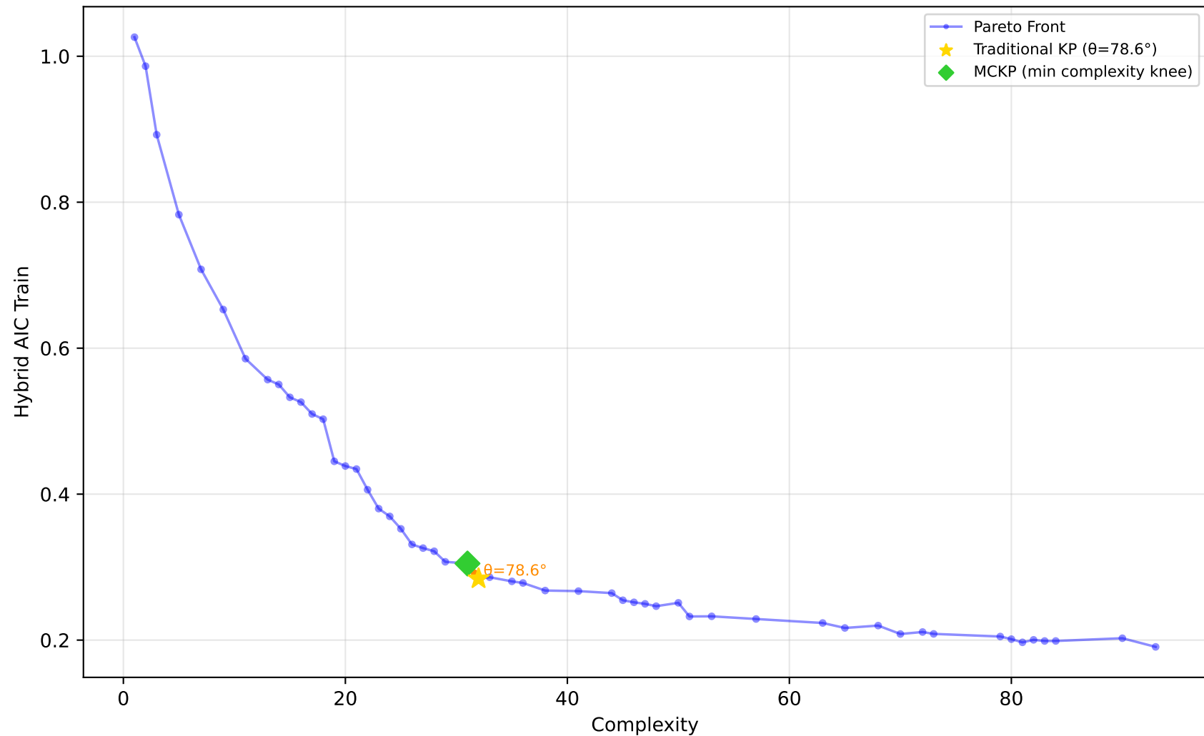
229_pwLinear - Run 3 - SVP - Hybrid AIC Train \lambda_1=0.50, \lambda_2=0.10, \lambda_3=0.00 | Difficulty: 1.00 | Method: hmr
