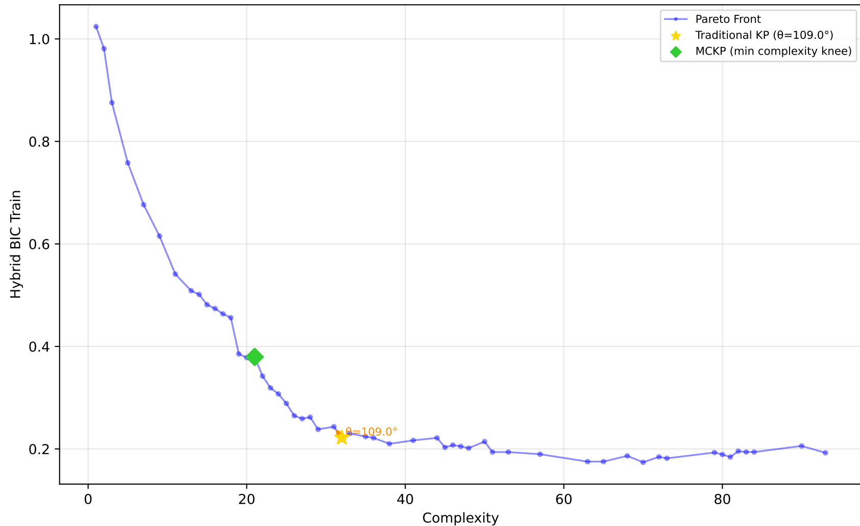
229_pwLinear - Run 3 - SVP - Hybrid BIC Train \lambda_1=0.50, \lambda_2=0.00, \lambda_3=0.00 | Difficulty: 1.00 | Method: hmr
