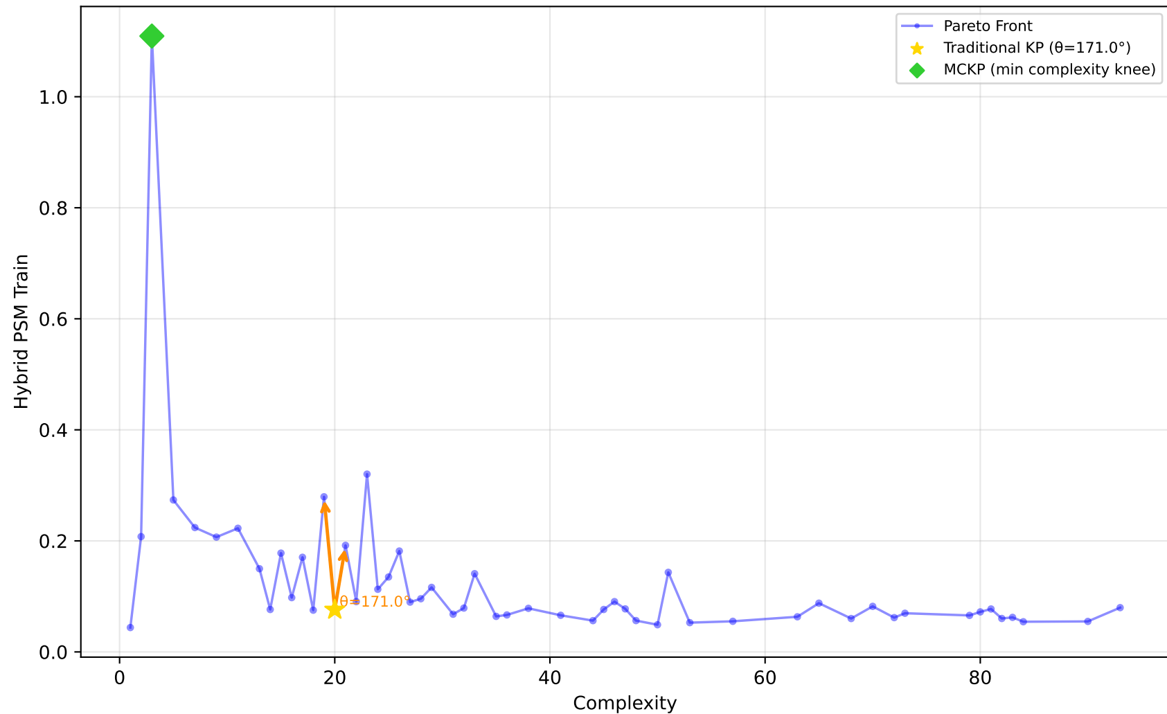
229_pwLinear - Run 3 - SVP - Hybrid PSM Train \lambda_1=0.50, \lambda_2=0.00, \lambda_3=0.00 | Difficulty: 1.00 | Method: hmr
