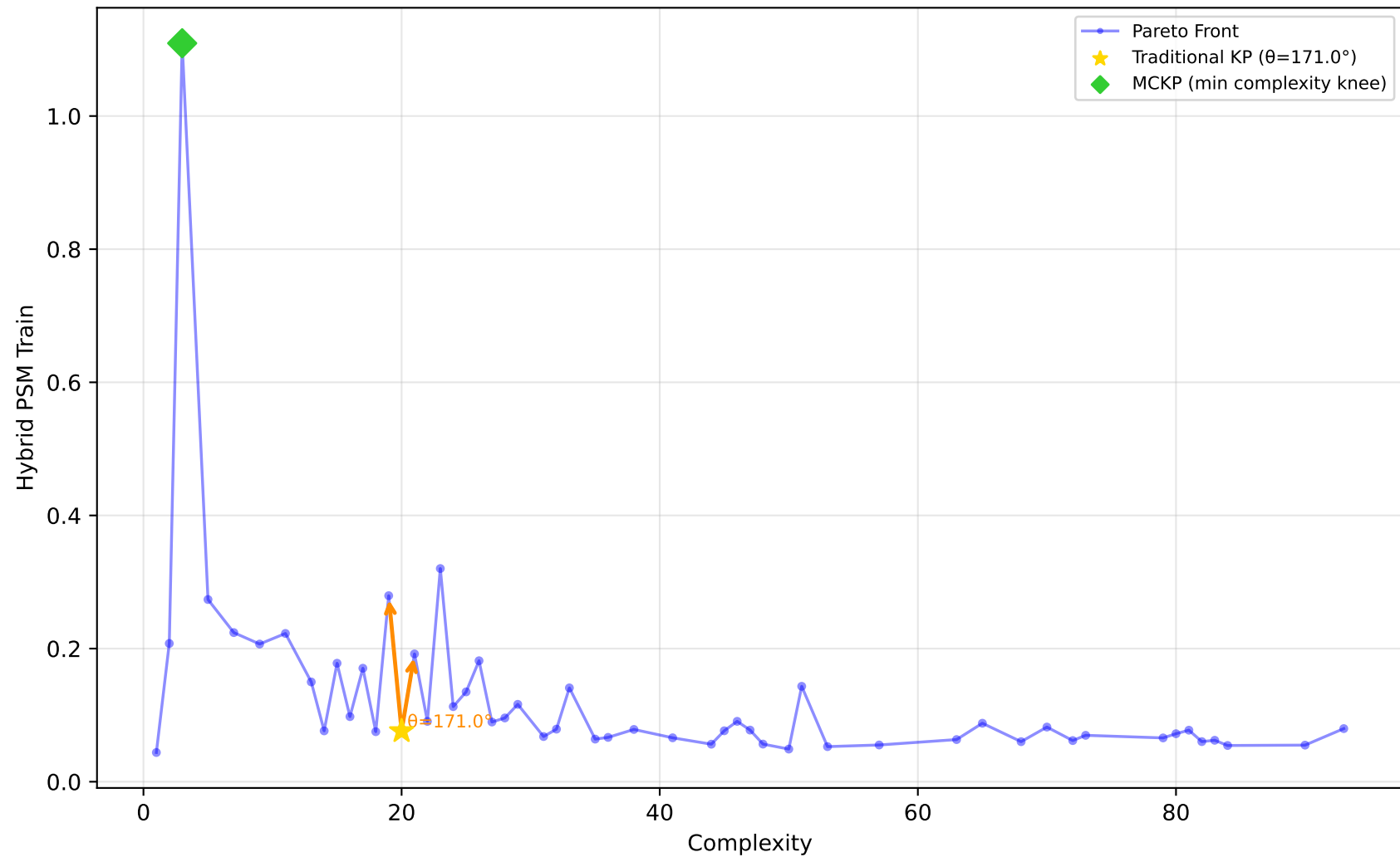
229_pwLinear - Run 3 - SVP - Hybrid PSM Train \lambda_1=0.50, \lambda_2=0.10, \lambda_3=0.00 | Difficulty: 1.00 | Method: hmr
