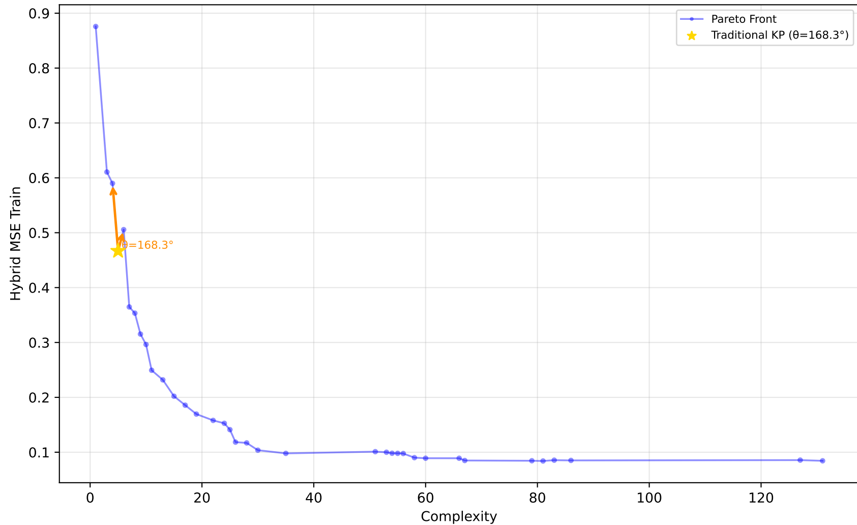
229_pwLinear - Run 4 - MVP - Hybrid MSE Train \lambda_1=0.50, \lambda_2=0.00, \lambda_3=0.00 | Difficulty: 1.00 | Method: hmr
