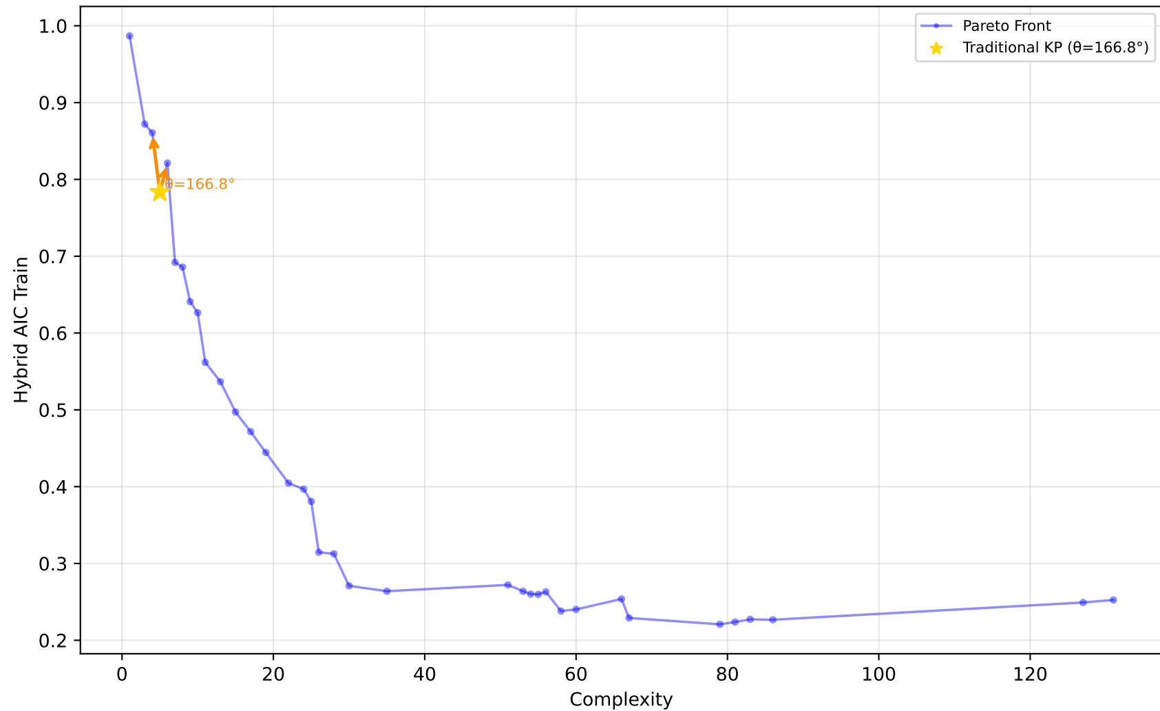
229_pwLinear - Run 4 - SVP - Hybrid AIC Train \lambda_1=0.50, \lambda_2=0.10, \lambda_3=0.00 | Difficulty: 1.00 | Method: hmr
