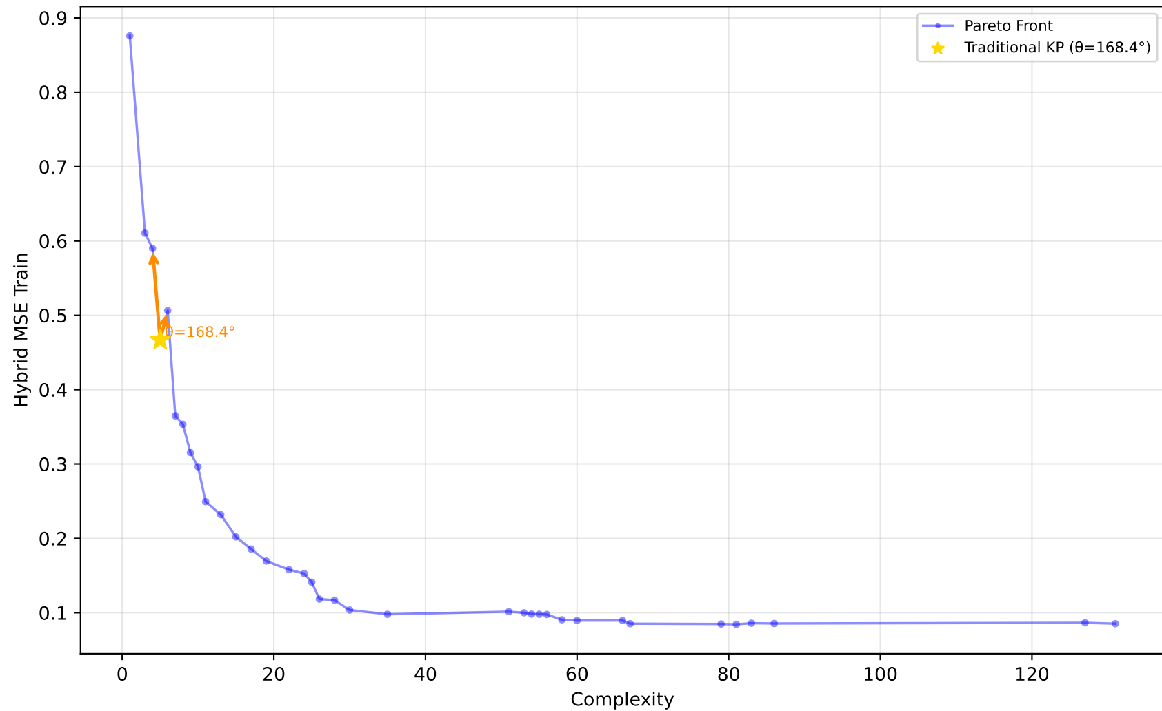
229_pwLinear - Run 4 - SVP - Hybrid MSE Train \lambda_1=0.50, \lambda_2=0.10, \lambda_3=0.00 | Difficulty: 1.00 | Method: hmr
