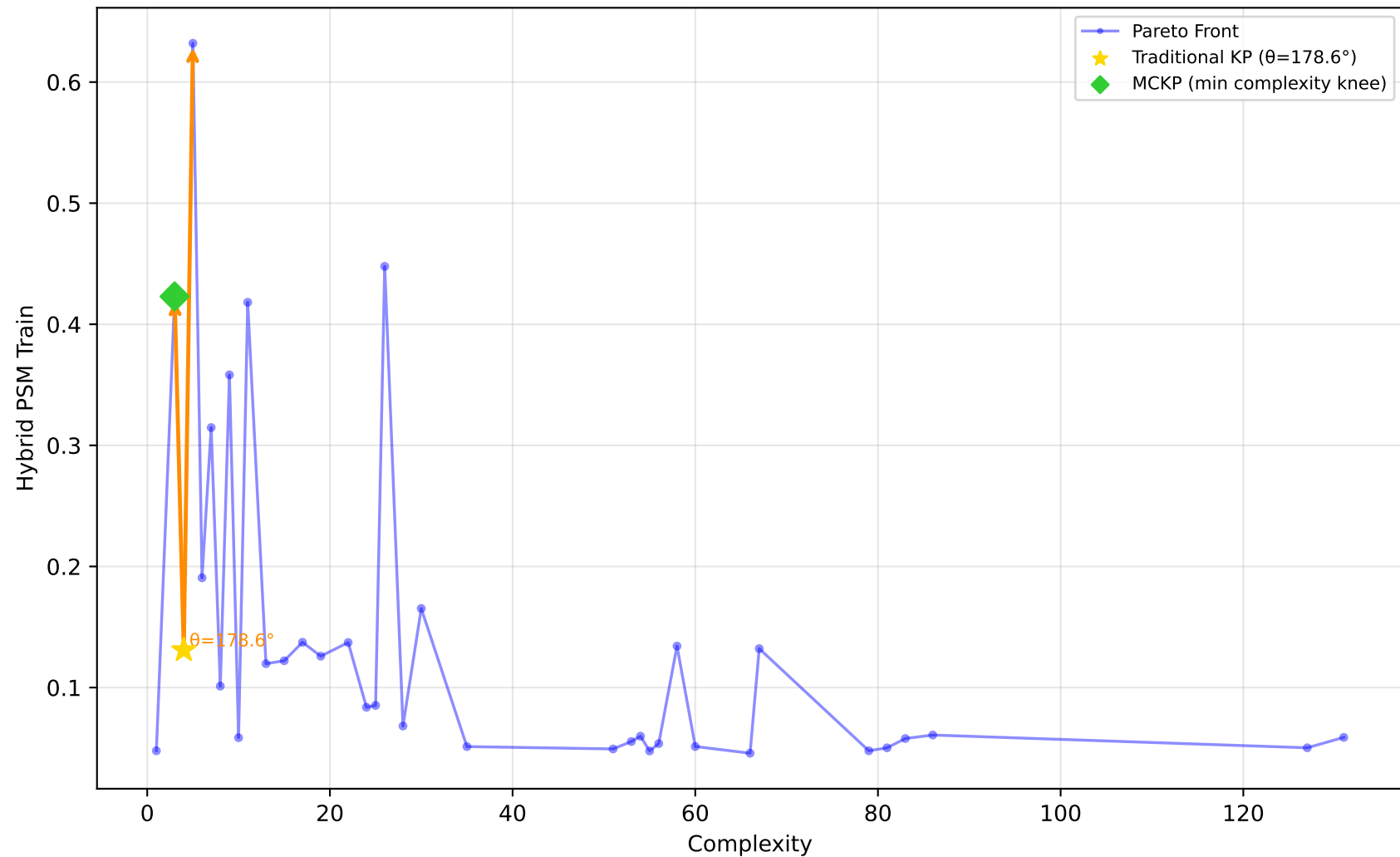
229_pwLinear - Run 4 - SVP - Hybrid PSM Train \lambda_1=0.50, \lambda_2=0.00, \lambda_3=0.00 | Difficulty: 1.00 | Method: hmr
