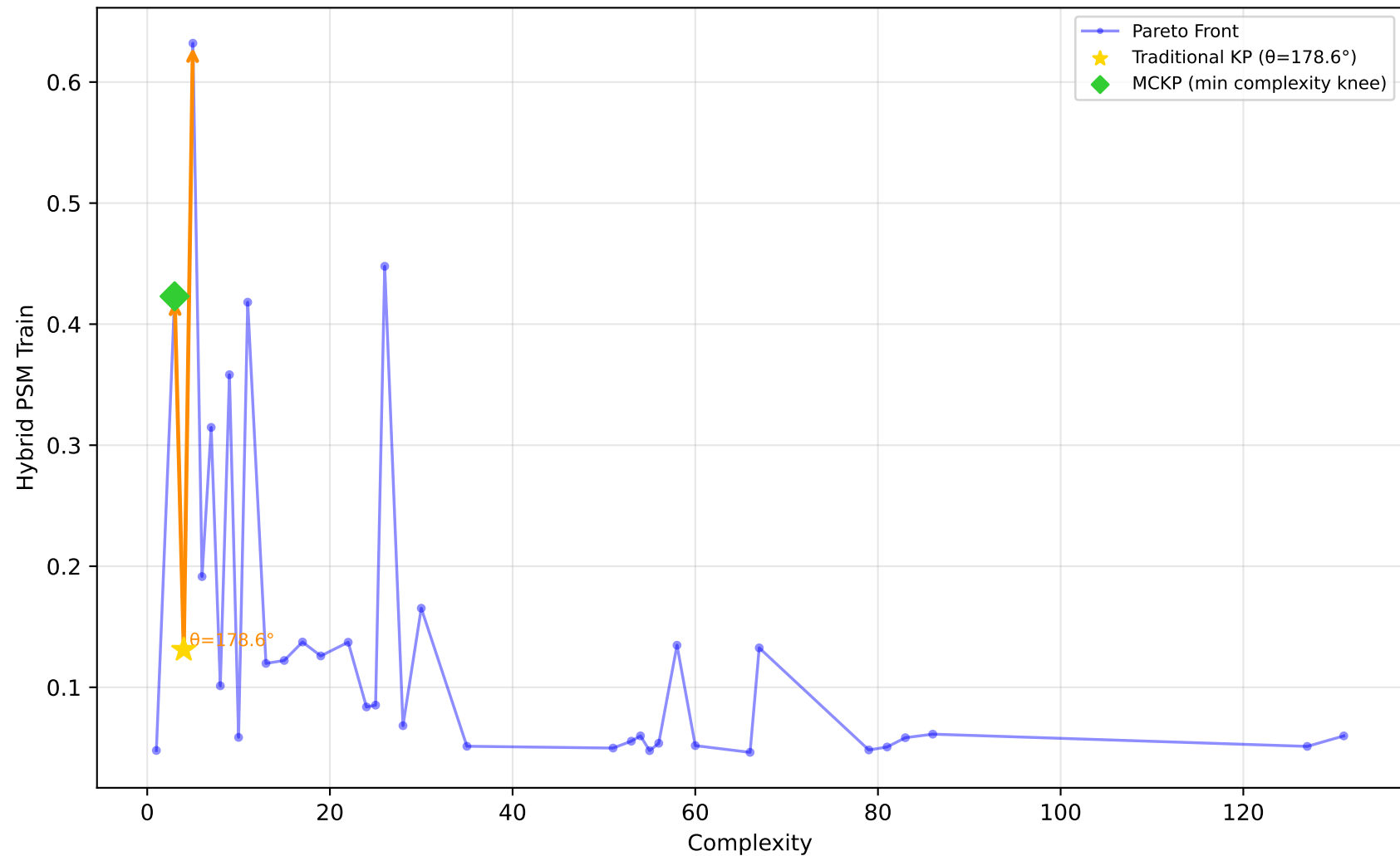
229_pwLinear - Run 4 - SVP - Hybrid PSM Train \lambda_1=0.50, \lambda_2=0.10, \lambda_3=0.00 | Difficulty: 1.00 | Method: hmr
