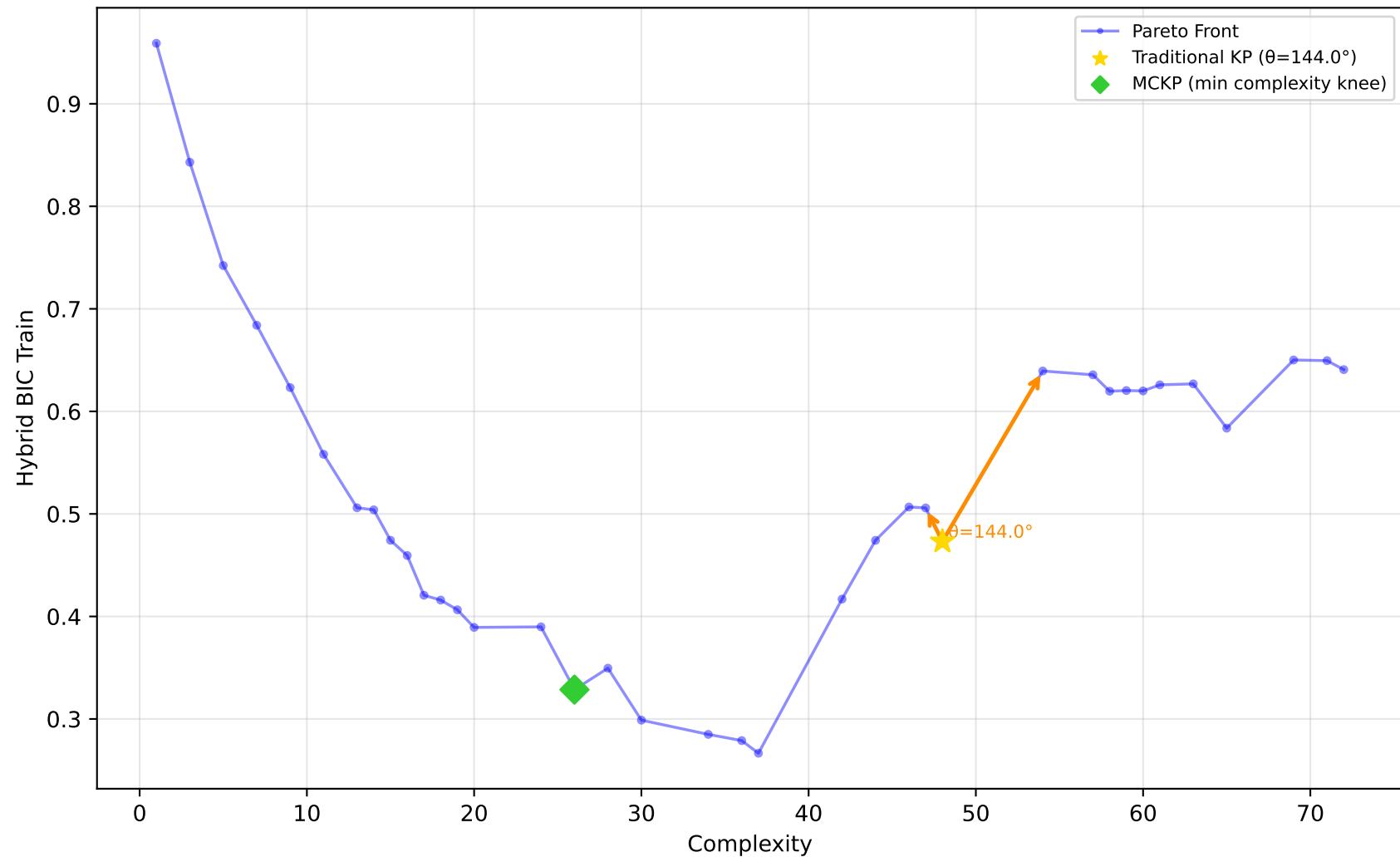
229_pwLinear - Run 5 - MVP - Hybrid BIC Train \lambda_1=0.50, \lambda_2=0.00, \lambda_3=0.00 | Difficulty: 1.00 | Method: hmr
